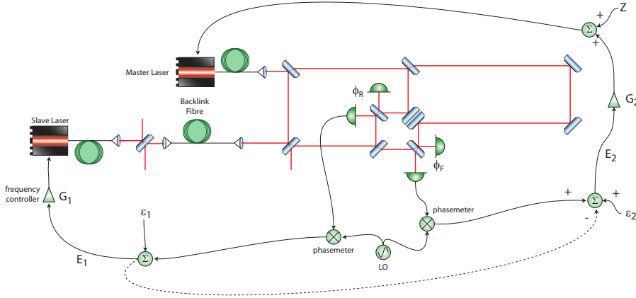
Figure 2. Simplified system layout. The interferometer readout labeled \phi_R exists in the current LISA optical bench design. The interferometer readout labeled \phi_F is the readout for the proposed additional interferometer for measuring and actively suppressing the laser frequency noise.
