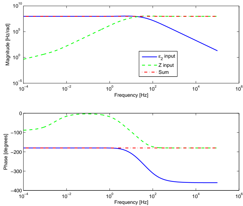
Figure 4. Frequency tuning response.
