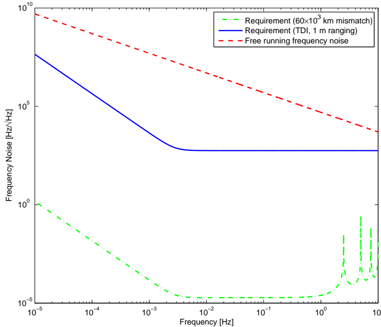
Figure 1. Frequency noise requirements for an arm length mismatch of 60 000 km ( 20 \mu\text{Hz}/\sqrt{\text{Hz}} at 0.1 Hz) and with TDI combined with 1 m ranging accuracy ( 560 \text{Hz}/\sqrt{\text{Hz}} at 0.1 Hz). Also shown for comparison is the typical free-running laser frequency for Nd:YAG NPRO lasers.
