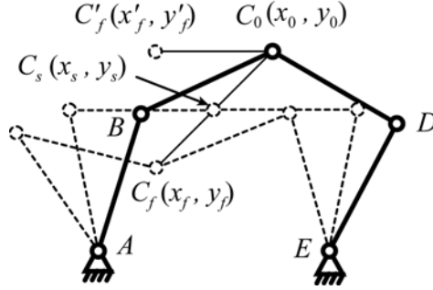
Figure 3. Initial, singular and final positions of the planar 5R parallel manipulator.
