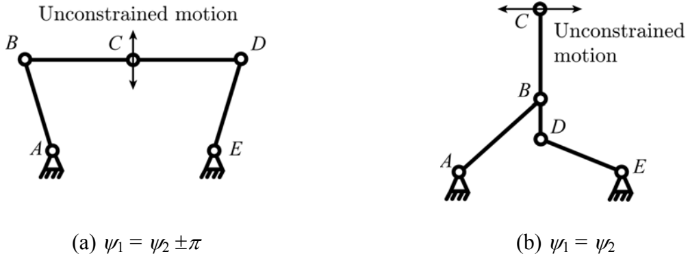
Figure 1. Kinematic chain of the planar 5R parallel manipulator.
