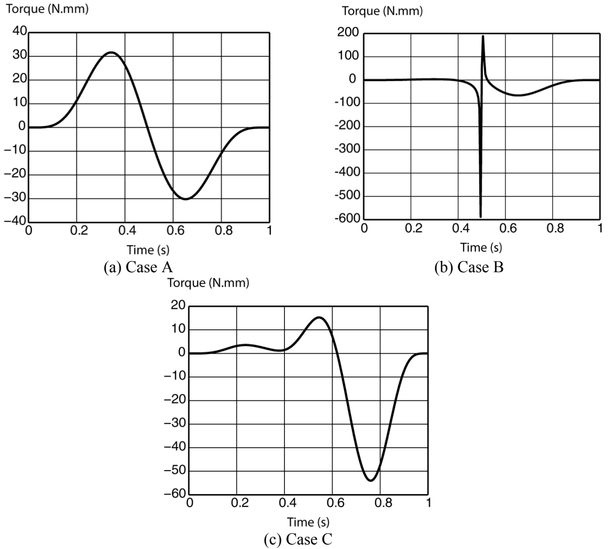
Figure 5. Torques values for the actuator 2.
