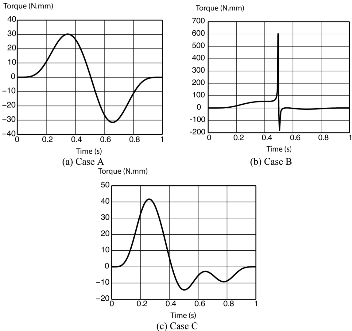
Figure 4. Torques values for the actuator 1.
