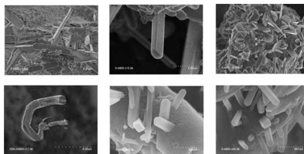
Fig. 4 Scanning electron microscopy images of B_{Ba^{2+}} hybrid material after the sol-gel step (bottom) and after the calcination step (lower).
