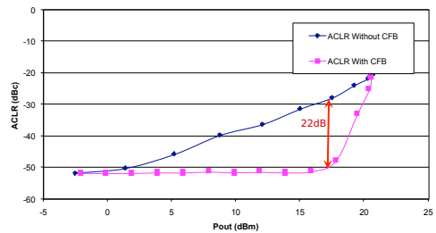
Fig. 5. ACPR at 5 MHz offset for W-CDMA signal in open and closed loop
