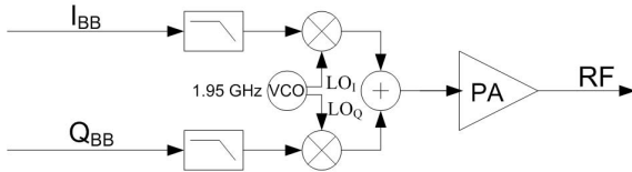
Fig. 2. Zero-IF Architecture
