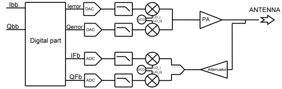
Fig. 3. Architecture of a Cartesian Feedback linearization technique
