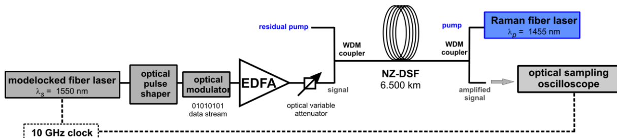
Figure 1. Experimental set-up.
