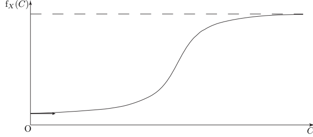
FIGURE 9. Graph of the function f_X .
