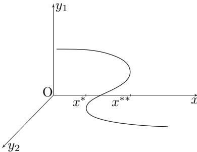
FIGURE 1. A hysteresis curve.
