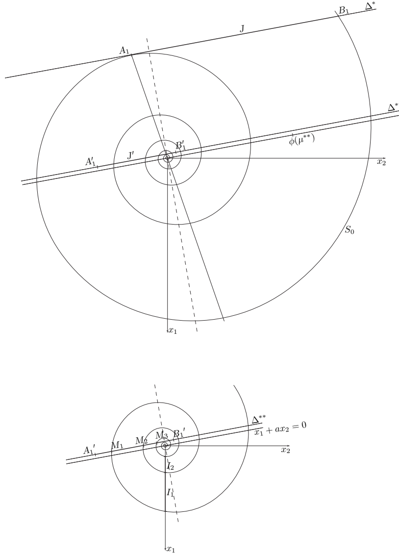
FIGURE 7. The one-dimensional section I covered twice by the flow \varphi_3 .
