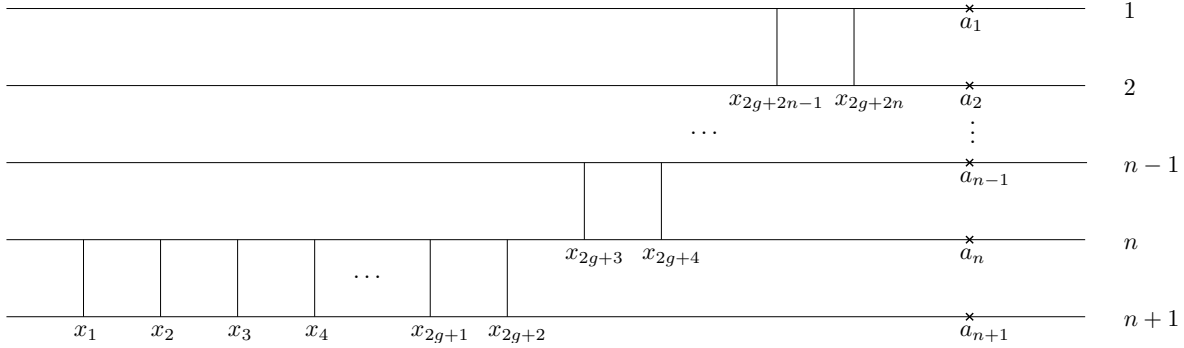
Figure 1: Hurwitz diagram of the covering \mathcal{R}_{g,n+1} .
