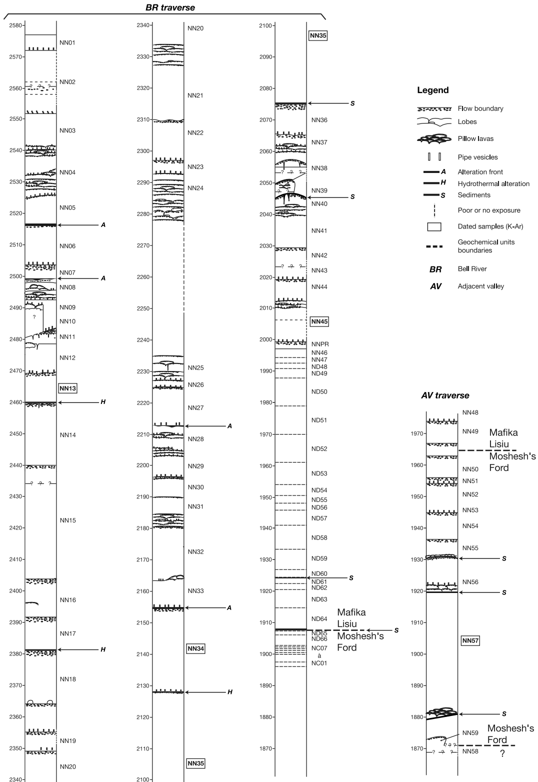
Figure 3. Stratigraphic log of the Naude's Nek section: main (BR) traverse and adjacent small valley (AV) traverse.
