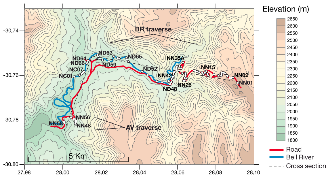
Figure 4. Location of the 88 paleomagnetic sites sampled along the BR and AV traverses. Topographic map is based on Shuttle Radar Topography Mission 2 (SRTM2) [Rodriguez et al. , 2005].
