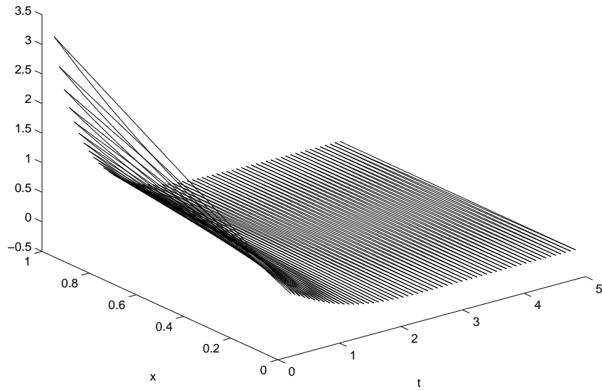
Figure 1. Approximated solution
