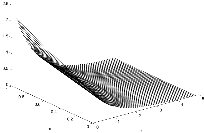
Figure 2: Exact solution
