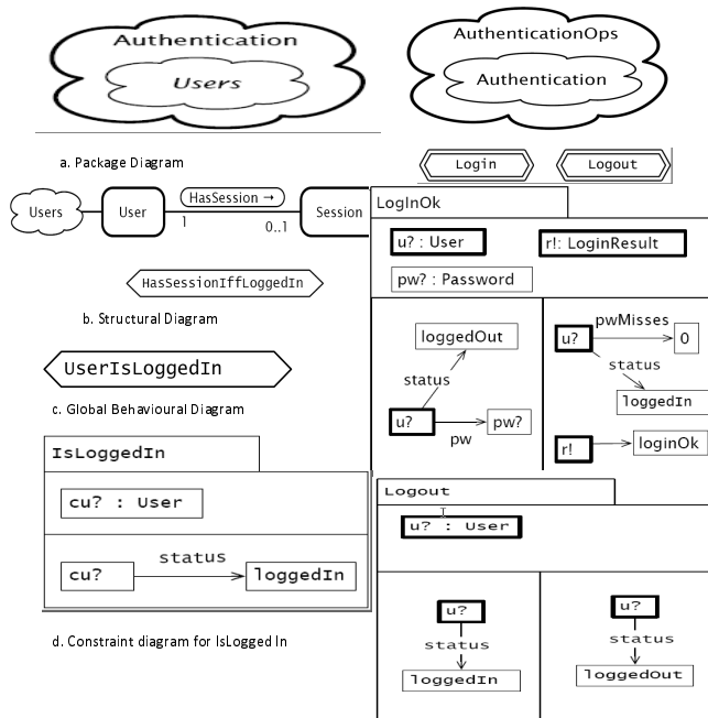
Fig. 11. VCL Packages Authentication and Authorization
