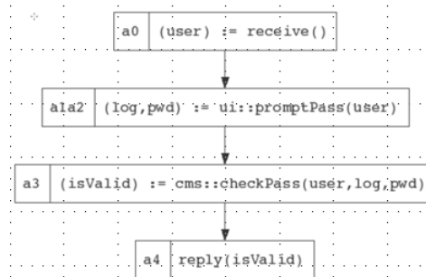
Fig. 8. Orchestration:cms:authUser
