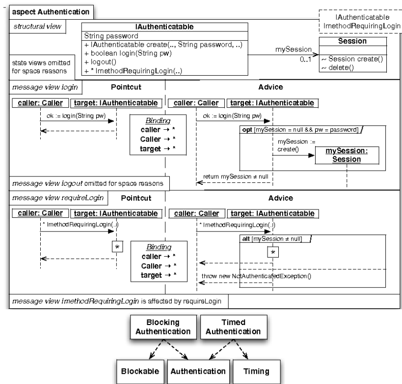
Fig. 3. RAM model
