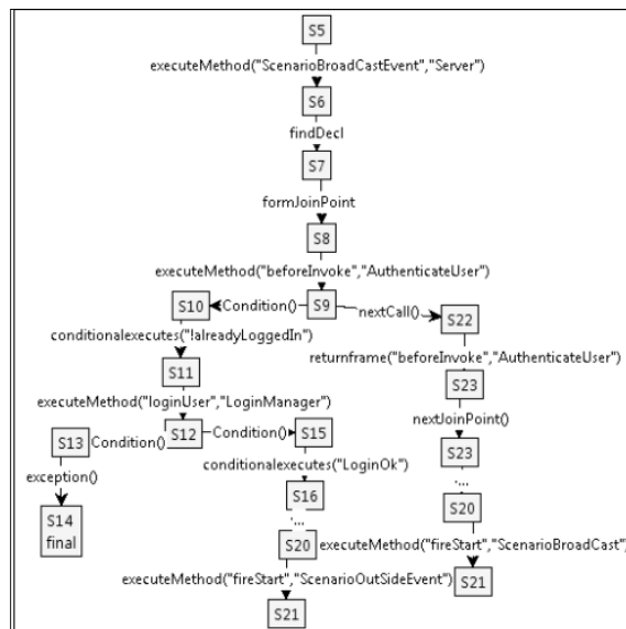
Fig. 6. GrACE:Execution tree
