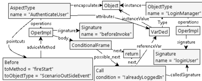
Fig. 5. GrACE:DSM Authenticate
