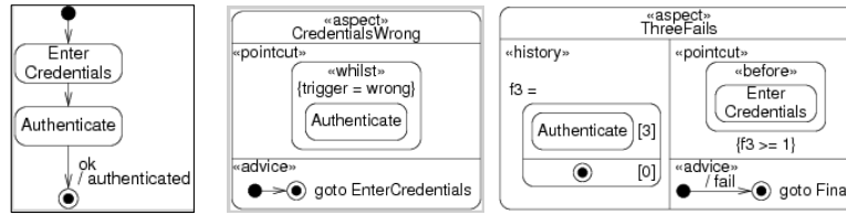
Fig. 7. HiLA model
