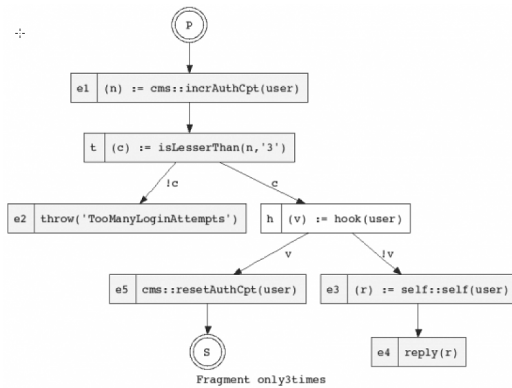
Fig. 9. Authentication concern in an ADORE model
