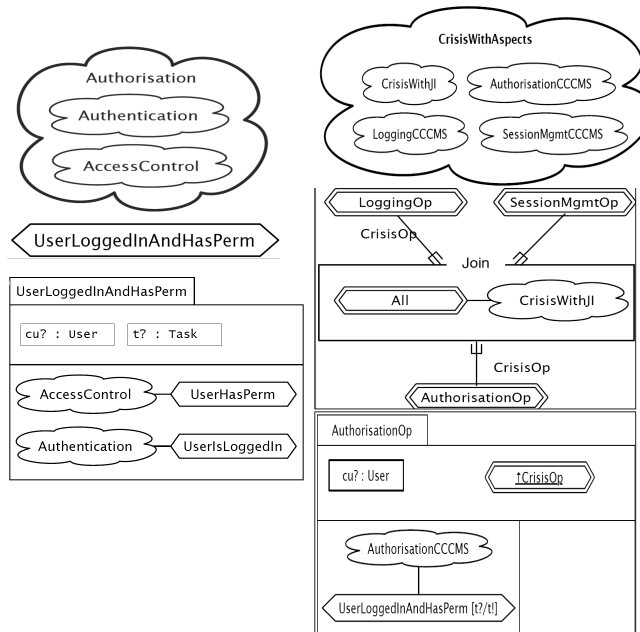
Fig. 12. VCL Packages Authorization and Crisis with Aspects
