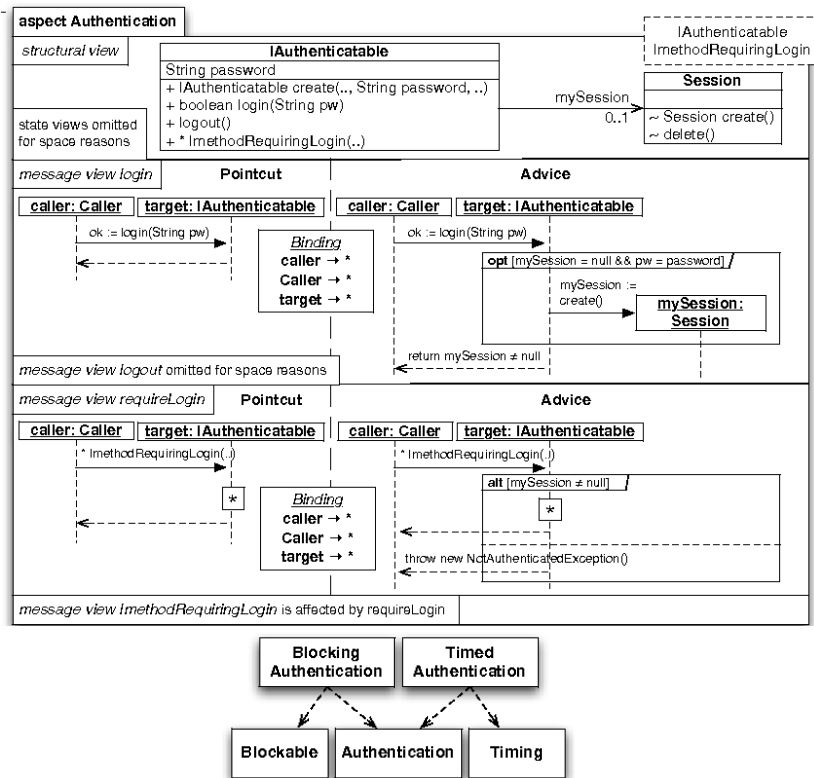
Fig. 3. RAM model
