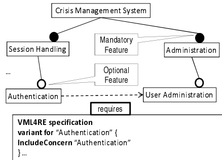
Fig. 1. VML4RE model
