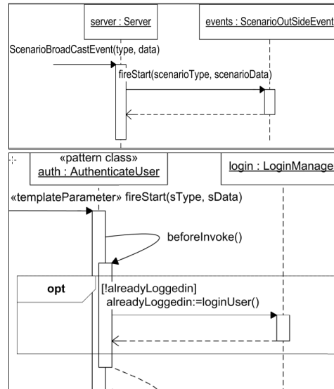
Fig. 4. GrACE:Sequence diagrams
