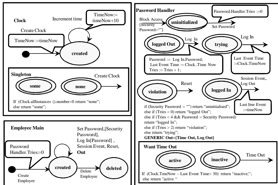
Fig. 10. Protocol Model of the Authentication Concern
