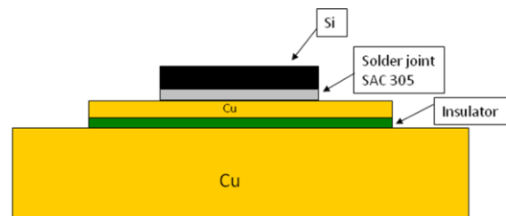
Figure 1 - Leadframe model
