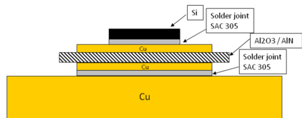
Figure 2 - DBC model
