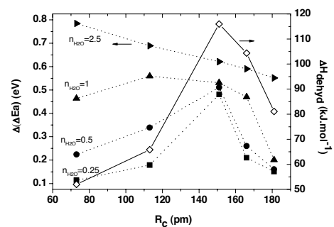
Fig.8: \Delta(\Delta E a) (see text for its definition) for various water loadings n_{H_2O} (left axis, symbols \alpha, \beta, \gamma for n_{H_2O} = 0.25; 0.5; 1 & 2.5 respectively) and \Delta H_{dehyd} , the dehydration enthalpy, (right axis, symbols M) as a function of the cation radius.
