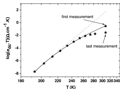
Fig. 6. logarithm of the product dc conductivity · temperature as function of the temperature (in reciprocal scale). Symbols are the experimental data. The dot line is the Arrhenian behavior (eq.1) calculated from the lowest measurement temperatures only. The full line correspond to the VTF fit (eq.2) considering the first measurement and all the measurement comprised between the lowest temperature and TT - 50\text{K} . See text for more details about the VTF fitting procedure. Case of the \text{Na}^+ -montmorillonite dehydrated at TT = 303\text{K} .
