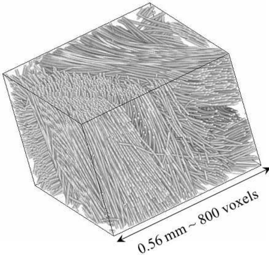
Fig. 3. Segmentation of C fibres in sample CC0 (raw preform) from an edge-detection tomograph. Resolution is 0.7\ \mu\text{m}/\text{voxel} . a) Slice of the original data set. b) 3D rendering.
