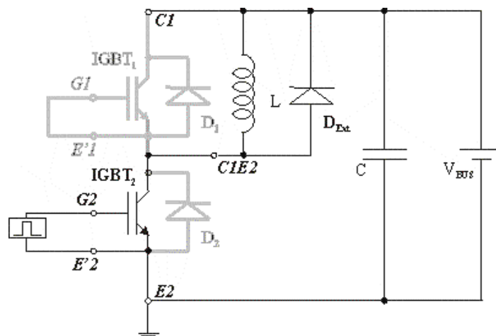
Figure 12 – Second version of the test circuit
