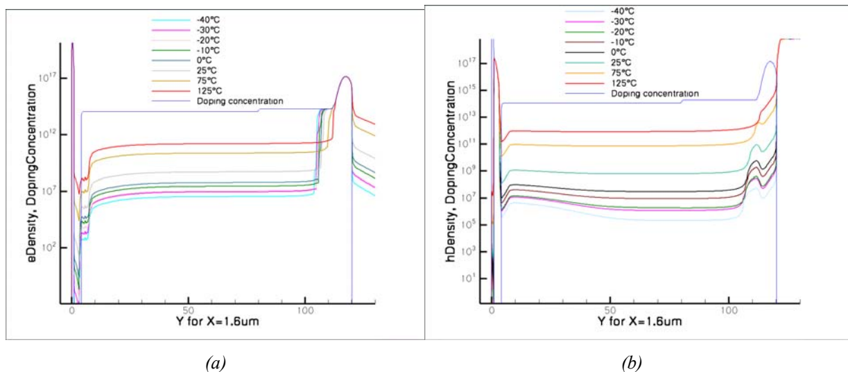
Figure 45 - (a) Electrons and (b) holes concentrations
