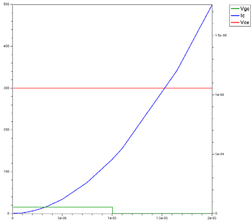
Figure 55 – Use of plugin: the simulation converge but the device does not switch
