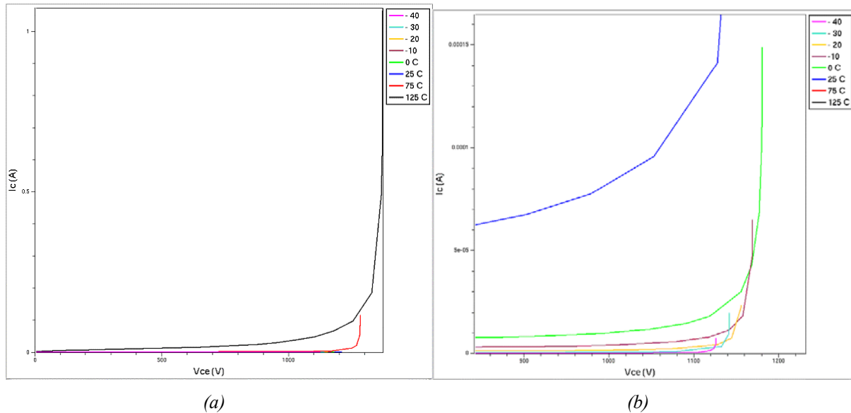
Figure 44 - (a) BVCEO curves (b) zoom for very low leakage currents
