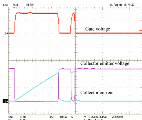
Fig. 8 - Full double-pulse configuration
