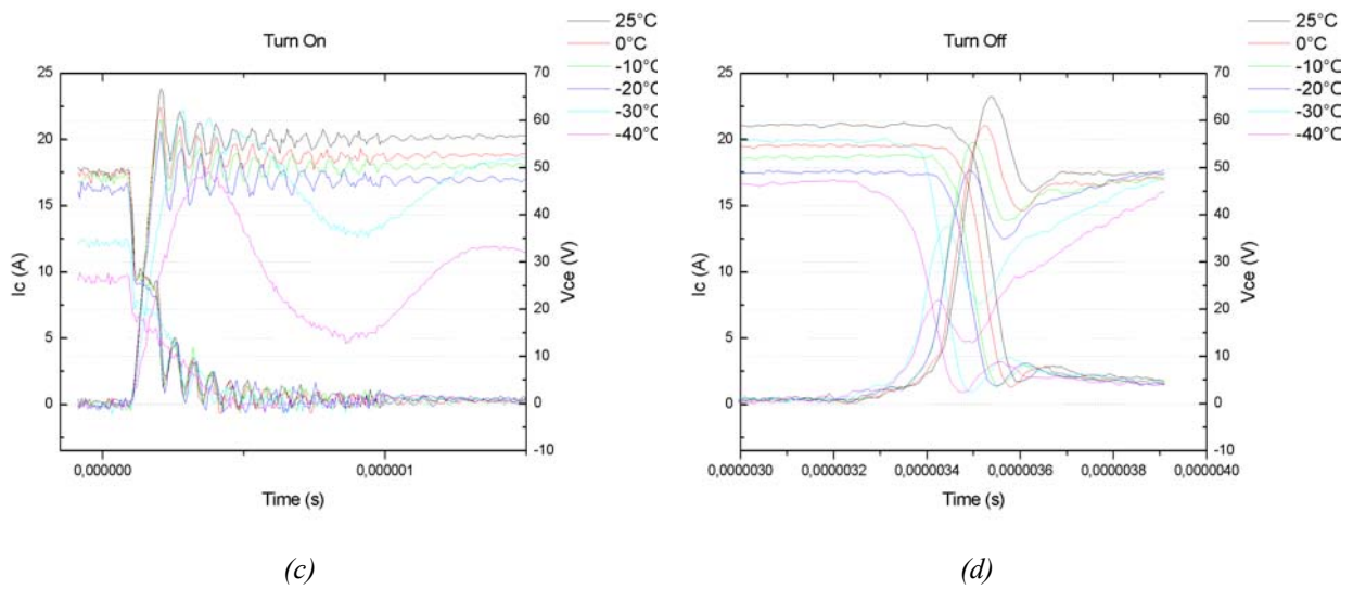
Figure 21 – Hard-switching for T = [25^{\circ}C \text{ down to } -40^{\circ}C] , R_g=2.2 \Omega and I_c=20A (a) full waveforms (b) on-state (c) turn-on and (d) turn-off
