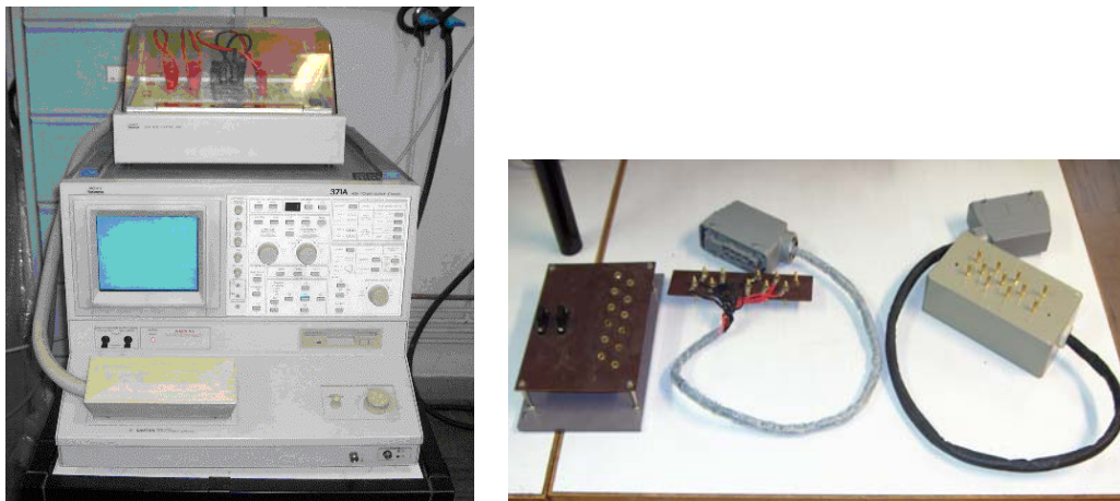
Figure 4 – Curve tracer and the specific cable for high and low temperature measurement
