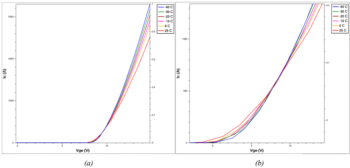
Figure 43 - (a) Ic-Vge curves (b) zoom for low Vge values
