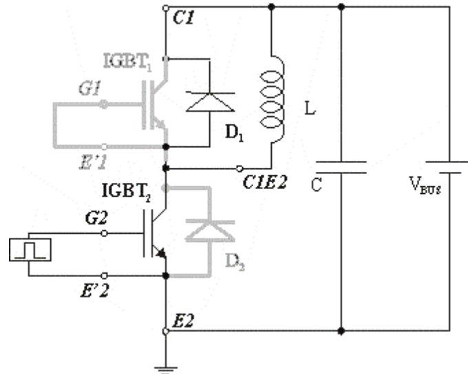
Figure 11 – First version of the test circuit
