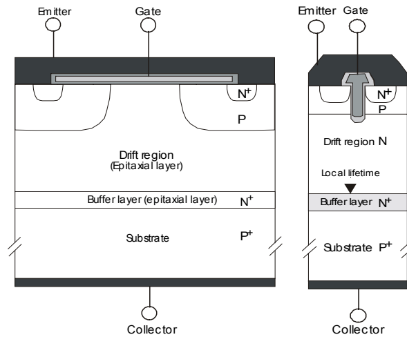
Figure 2 - Devices structure of P- and T-IGBTs
