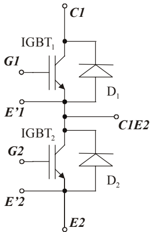
Fig.2 – Single-leg inverter power module arrangement
