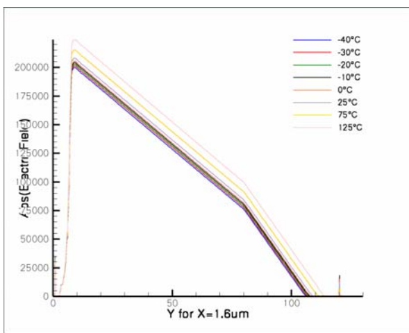
Figure 46 - Electric field
