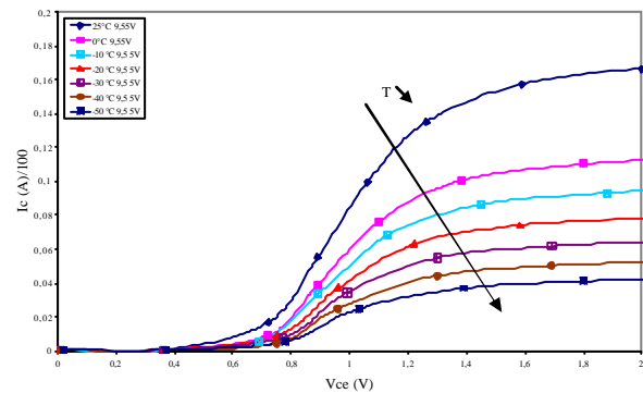
Fig.8 – I_c - V_{ce} characteristics for T = [25^{\circ}\text{C down to } -50^{\circ}]
