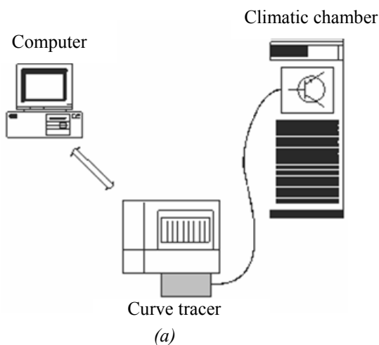
Figure 5 – Description of the complete static test bench (a) schematics and (b) photo
