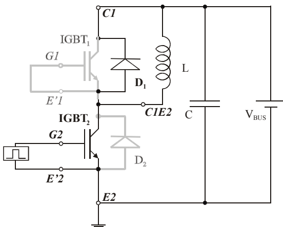
Fig.3 – First version of the test circuit
