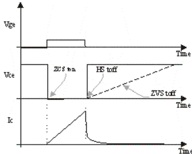
Figure 15 – Single-pulse configuration
