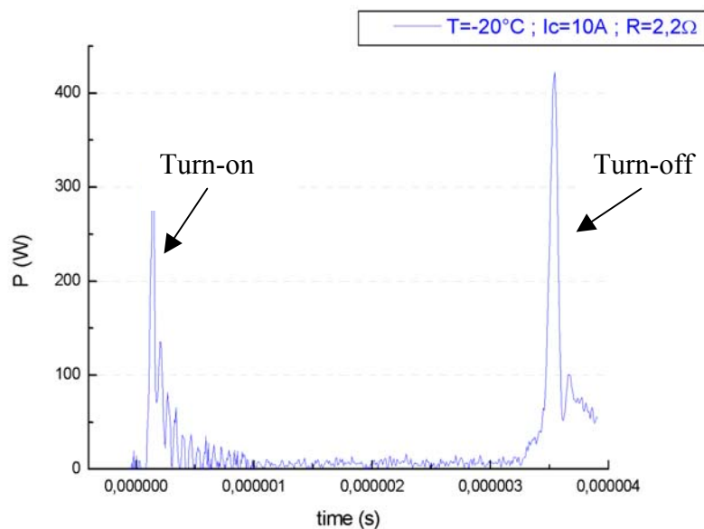
Figure 36 – Instantaneous peak power during transient for T = -20^\circ\text{C} , I_c = 10\text{A} and R_g = 2.2\ \Omega
