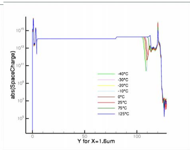
Figure 47 - Space charge within the device
