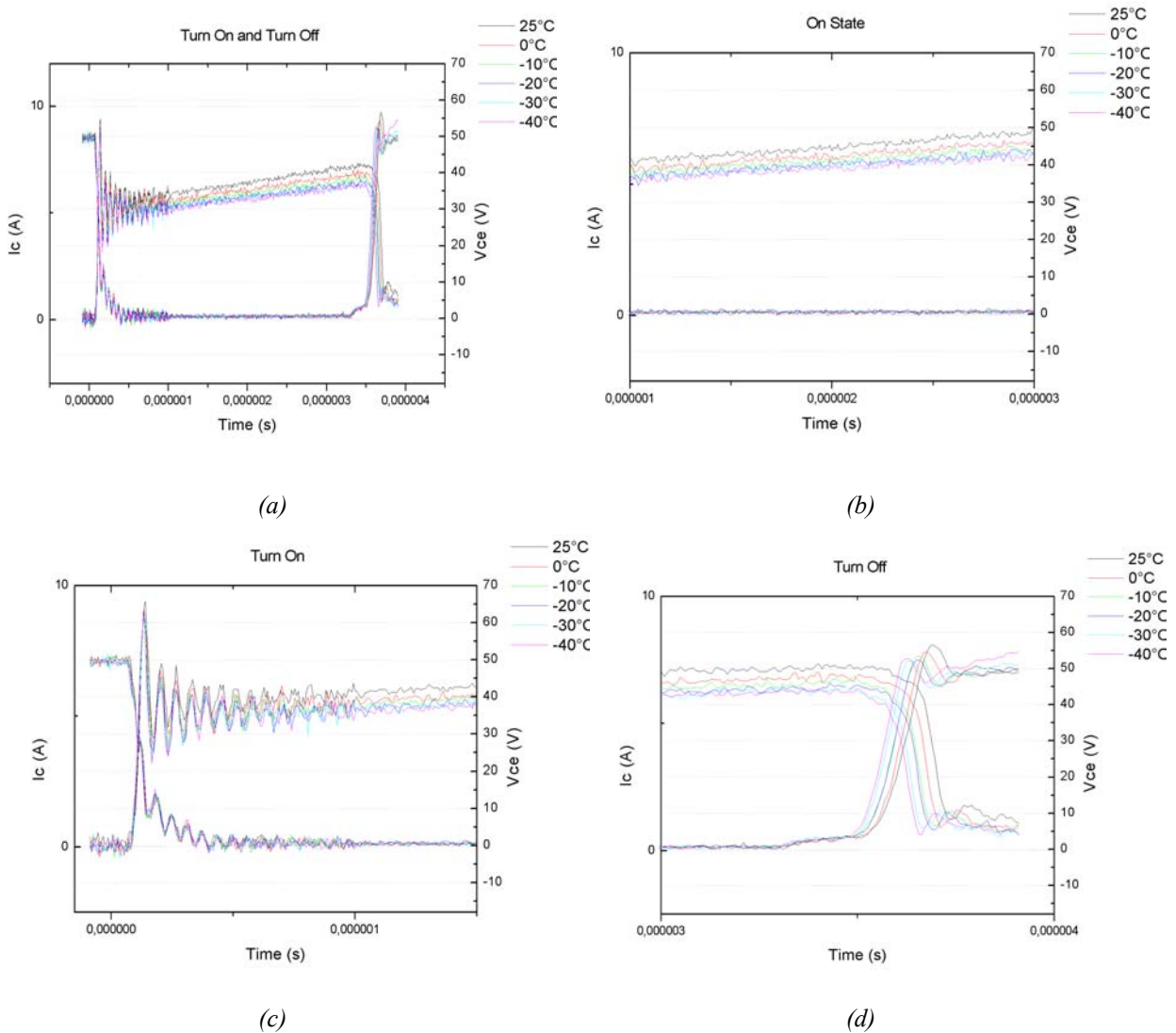
Figure 18 – Hard-switching for T = [25^{\circ}\text{C down to } -40^{\circ}\text{C}] , R_g=2.2\ \Omega and I_c=5\text{A} (a) full waveforms (b) on-state (c) turn-on and (d) turn-off
