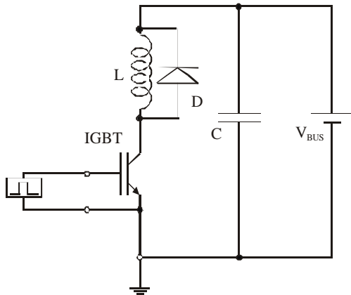
Fig.3 – Hard-switching test circuit [8]
