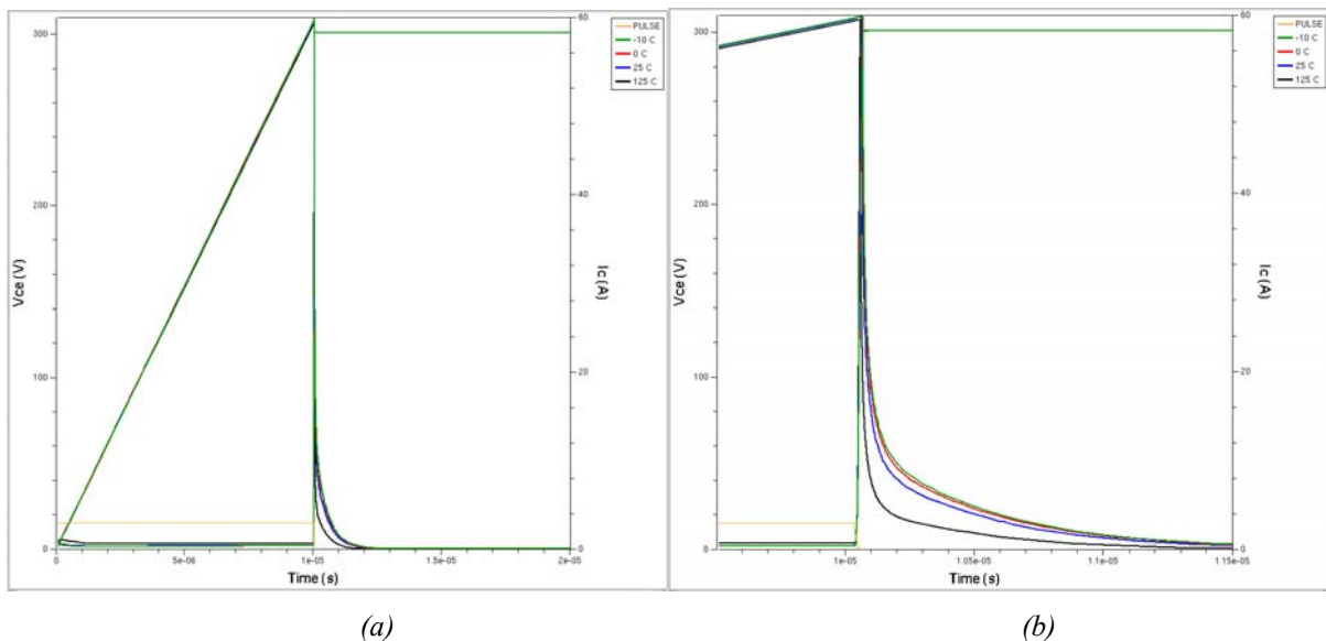
Figure 53 - “Strange” turn-off at various temperature (a) full waveforms (b) zoom on turn-off
