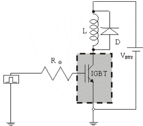
Figure 51 - Inductive load single gate pulse switching test circuit (in grey the 2D IGBT structure)
