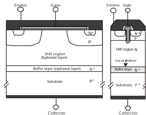
Fig.1 – Structure of the Planar and Trench punch through IGBTs
