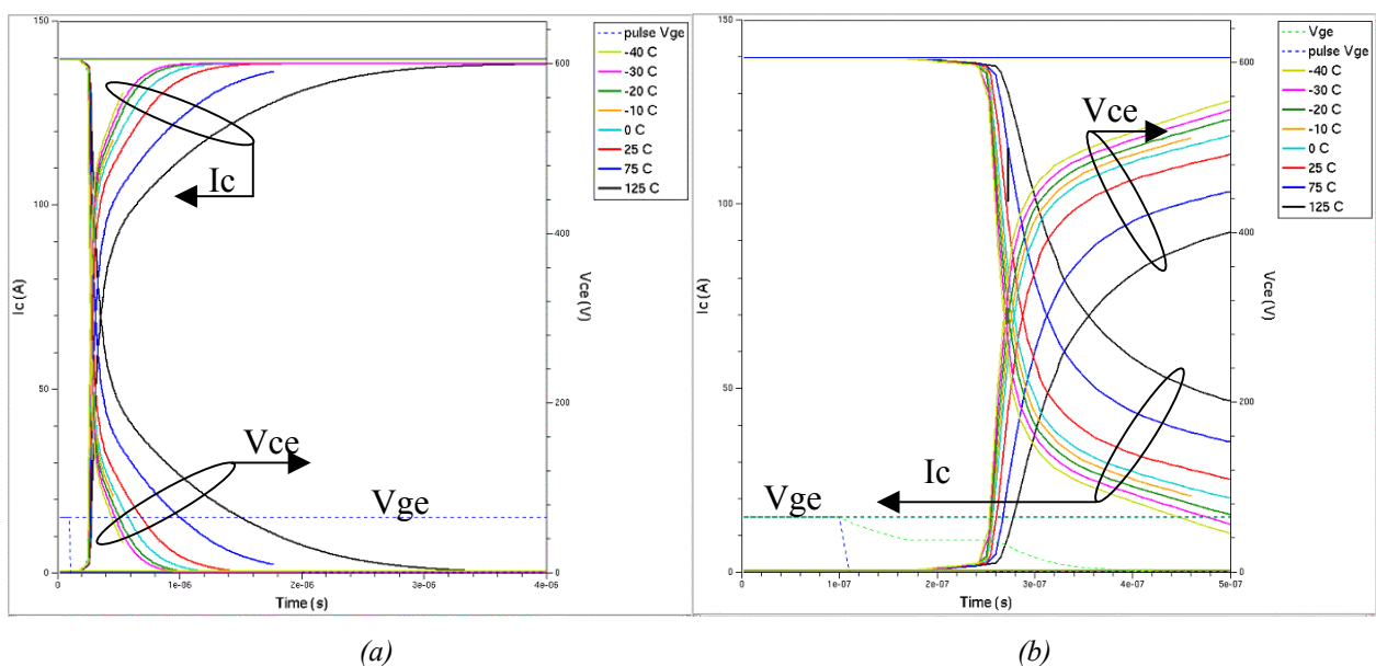
Figure 50 - Current and voltage waveforms under resistive load for (a) turn-on and (b) turn-off
