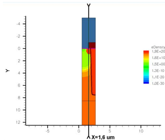
Figure 40 - xx' cutline for 1D analysis (zoom on the upper part of the device)
