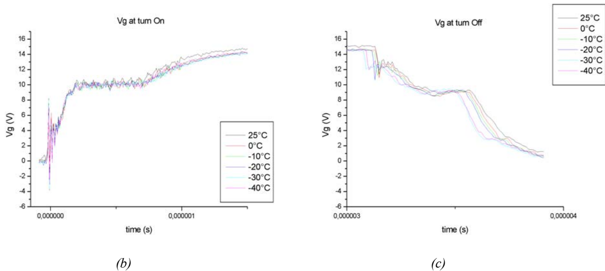
Figure 33 – Hard-switching for T = [25^{\circ}\text{C down to } -40^{\circ}\text{C}] , R_g=4.7 \Omega and I_c=20A (a) full waveforms (b) turn-on and (c) turn-off
