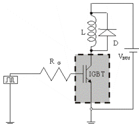
Figure 56 - Inductive load double gate pulse switching test circuit (in grey the 2D IGBT structure)
