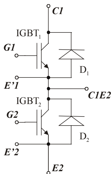
Figure 10 – Single-leg inverter power module arrangement
