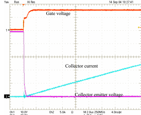
Fig. 9 - Zero-current switching turn-on
