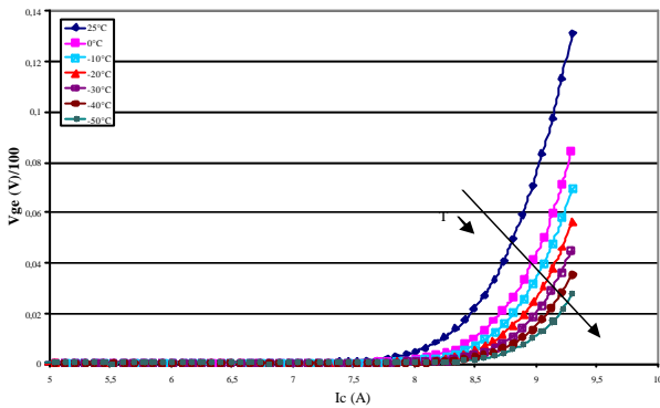
Fig.7 – I_c - V_{ge} characteristics for T = [25^{\circ}\text{C down to } -50^{\circ}]
