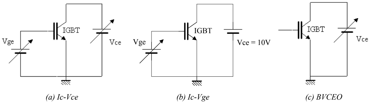
Figure 39 - Basic test circuits for static simulations
