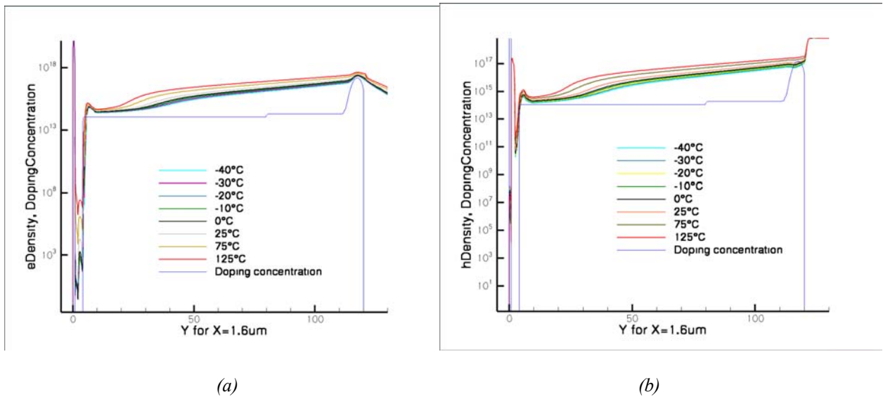
Figure 42 - (a) Electrons concentration (b) holes concentration
