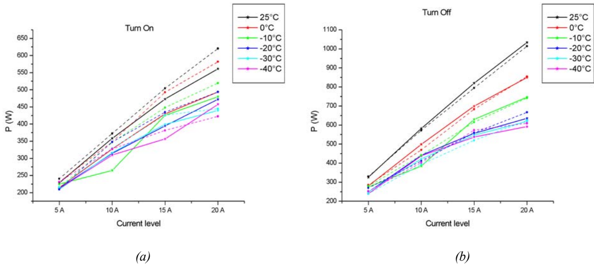
Figure 38 – Influence of the current load on the instantaneous peak power losses (a) turn-on (b) turn-off The dash lines correspond to R_g = 4.7 \Omega and the full line to R_g = 2.2 \Omega
