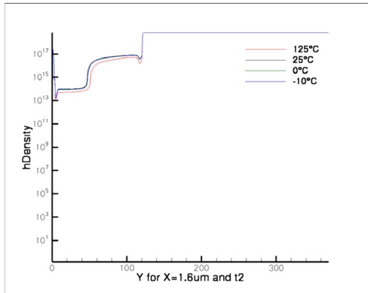
Figure 54 - Holes concentration at time t_2 for different temperature values
