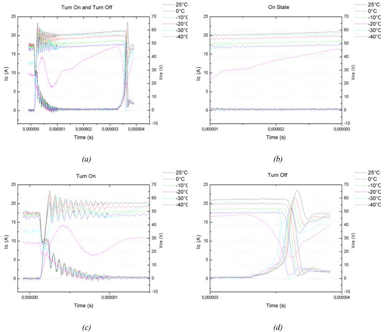
Figure 25 – Hard-switching for T = [25^\circ C \text{ down to } -40^\circ C] , R_g = 4.7 \Omega and I_c = 20A (a) full waveforms (b) on-state (c) turn-on and (d) turn-off
