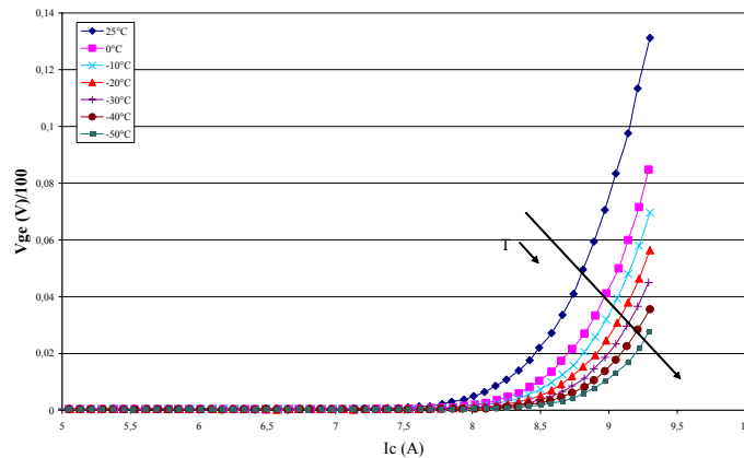
Figure 7 – Ic- Vge characteristics for T = [25^{\circ}\text{C down to } -50^{\circ}\text{C}]
