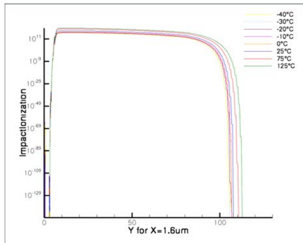
Figure 48 - Carriers generation by impact
