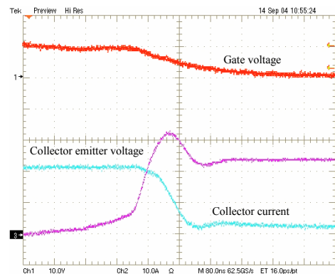
Fig. 11 - Hard-switching turn-off
