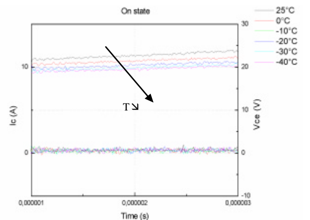
Fig.10 – Hard-switching on-state for T = [25^{\circ}\text{C down to } -40^{\circ}]
