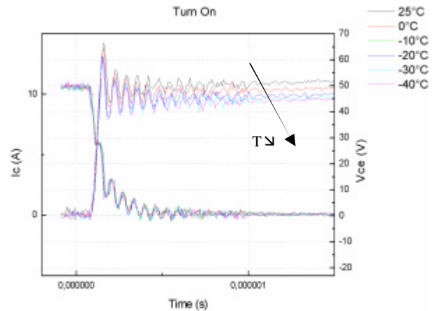
Fig.9 – Hard-switching turn-on for T = [25^{\circ}\text{C down to } -40^{\circ}]
