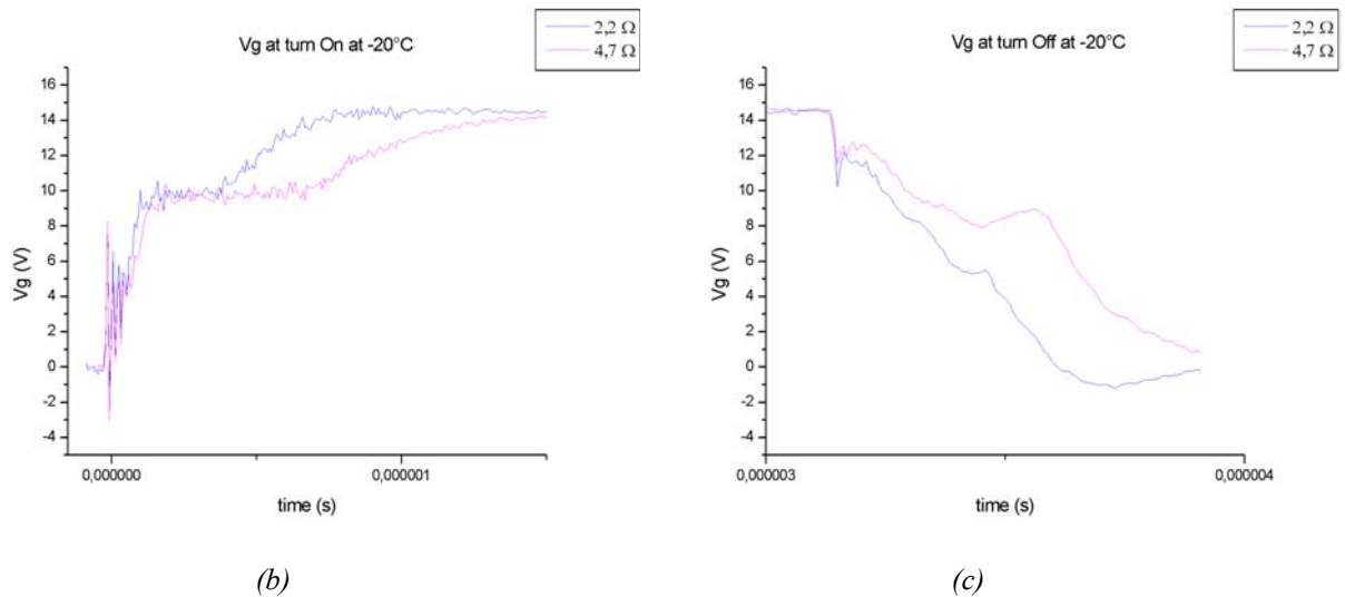
Figure 35 – Hard-switching for R_g = [2.2\ \Omega \text{ and } 4.7\ \Omega] , I_c = 15\text{A} and T = -20^\circ\text{C} (gate-emitter voltage)
