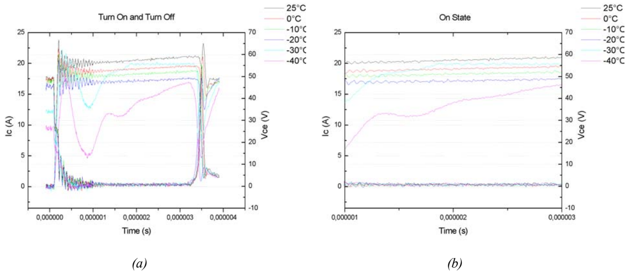
Figure 20 – Hard-switching for T = [25^{\circ}C \text{ down to } -40^{\circ}C] , R_g=2.2 \Omega and I_c=15A (a) full waveforms (b) on-state (c) turn-on and (d) turn-off
