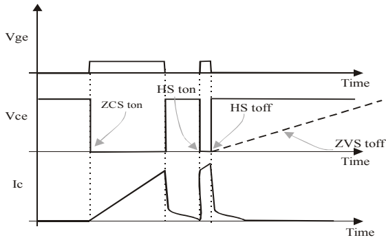
Fig. 7 - Double-pulse configuration
