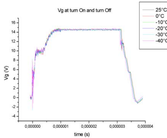
Figure 26 – Hard-switching for T = [25^{\circ}\text{C down to } -40^{\circ}\text{C}] , R_g=2.2 \Omega and I_c=5A (a) full waveforms (b) turn-on and (c) turn-off
