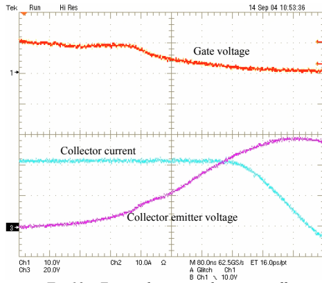
Fig.12 – Zero-voltage switching turn-off
