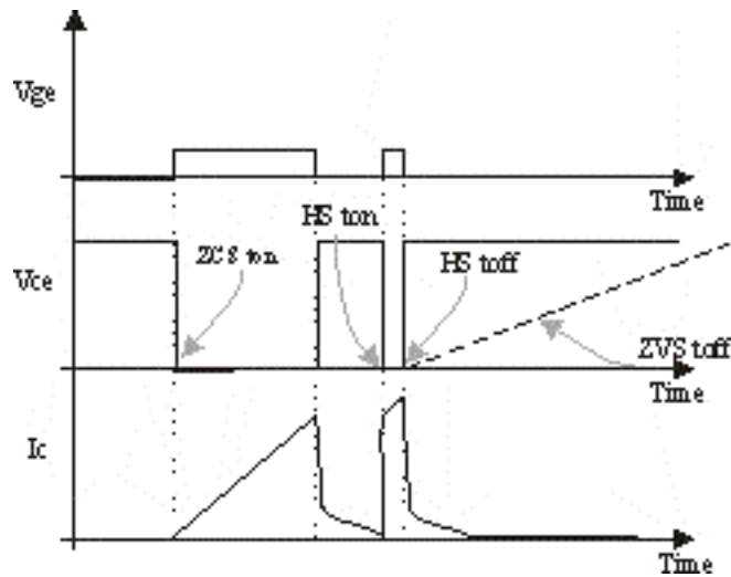
Figure 16 – Double-pulse configuration
