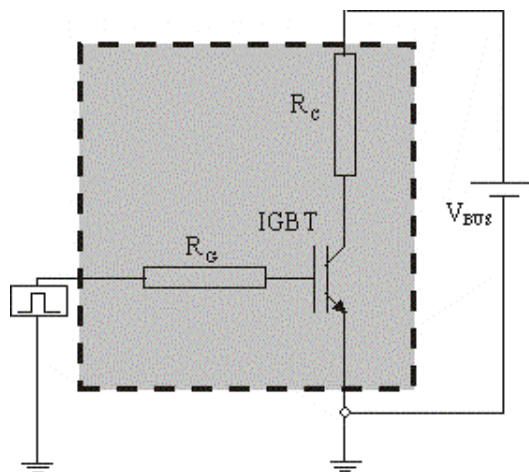
Figure 49 - Resistive load switching test circuit (in grey the 2D IGBT structure)
