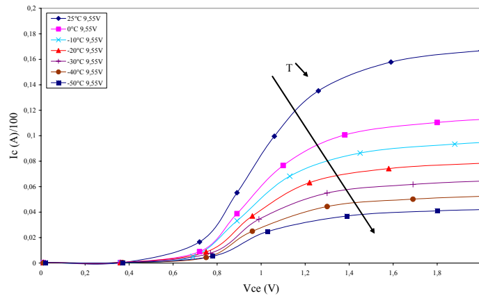
Figure 8 – I_c - V_{ce} characteristics for T = [25^{\circ}\text{C down to } -50^{\circ}\text{C}]
