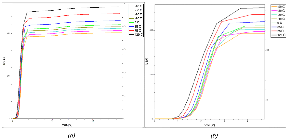
Figure 41 - (a) I_c - V_{ce} curve (b) zoom for low V_{ce} values
