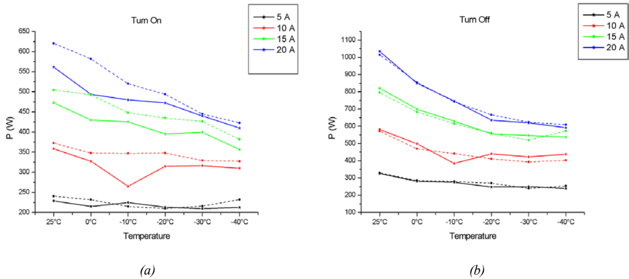
Figure 37 – Influence of the temperature on the instantaneous peak power losses (a) turn-on (b) turn-off The dash lines correspond to R_g = 4.7 \Omega and the full line to R_g = 2.2 \Omega
