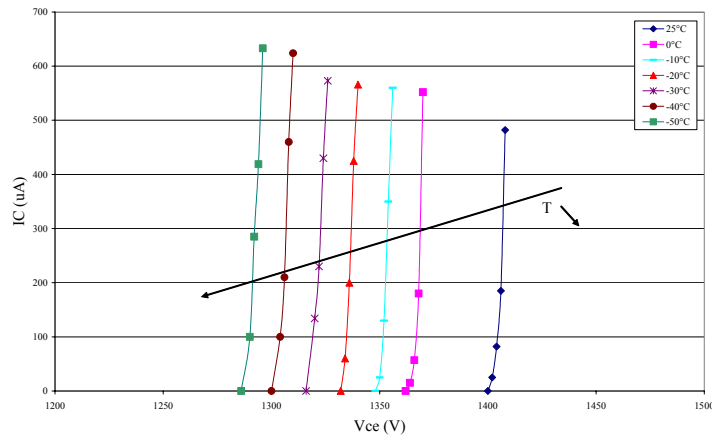
Figure 6 – BVCEO characteristics for T = [25^{\circ}\text{C down to } -50^{\circ}\text{C}]
