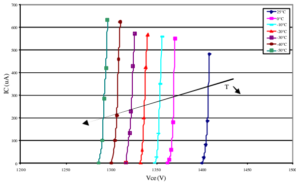
Fig.6 – BVCEO characteristics for T = [25^{\circ}\text{C down to } -50^{\circ}]
