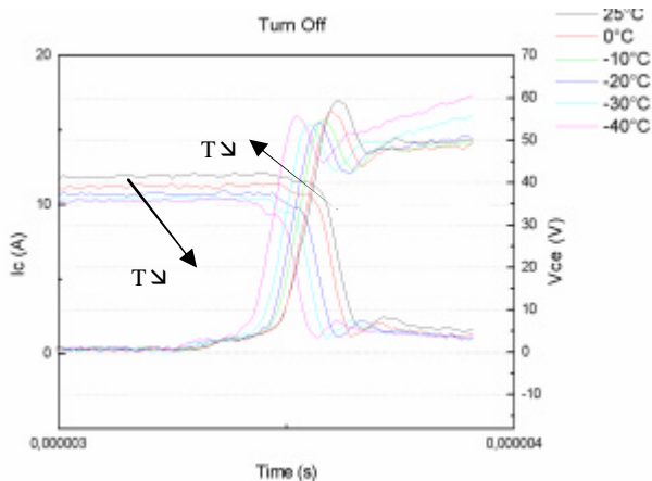
Fig.11 – Hard-switching turn-off for T = [25^{\circ}\text{C down to } -40^{\circ}]
