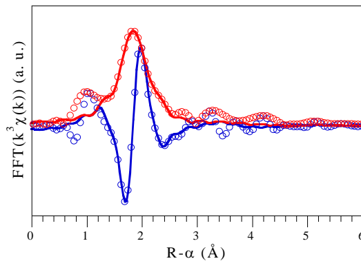
Fig. 3. Fit (solid lines) to the EXAFS (open circles) of the 6 wt. % Nd 2 O 3 parent glass (Nd-L 3 edge, room temperature).
