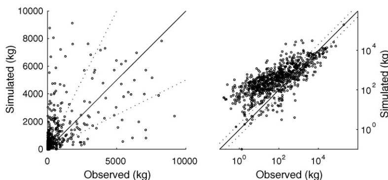
Fig. 7. Observed versus simulated suspended sediment fluxes on standard (left panel—for values up to 10,000 kg) and logarithmic (right panel) scales with the 3-7-1 MLP using Q , F^* and \Delta Q as inputs. The dashed lines delimit errors smaller than 100%.
