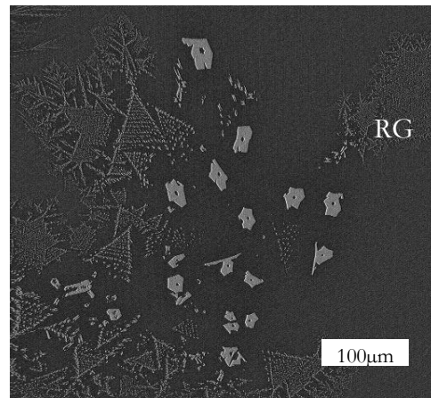
Figure 3 : Back-scattered SEM image of the neodymium bearing glass showing silicate apatite crystals with different microstructures formed during slow cooling of the melt (1°C/min); RG: residual glass.
