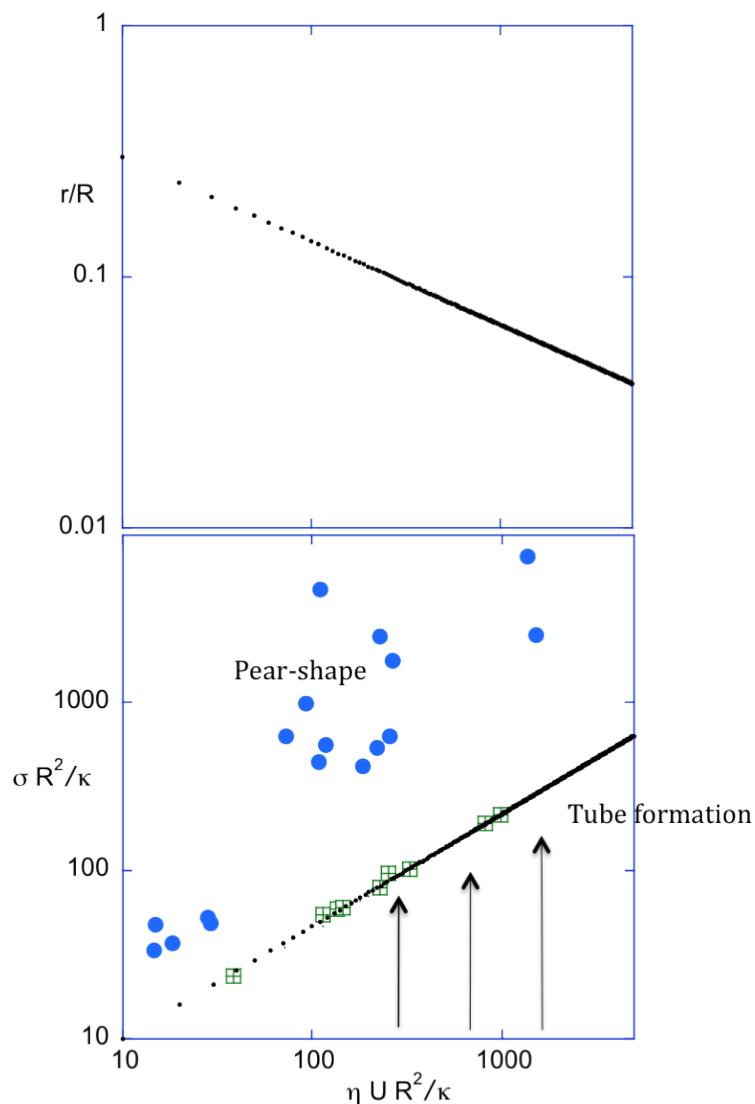
Figure 7 Theoretical curves (small dots) of variation of the ratio of the tube radius to the vesicle radius and of the adimensioned tension, \sigma R^2/\kappa as a function of the adimensioned capillary number \eta U R^2/\kappa for a vesicle drawing a tube. Filled circles correspond to pearlike vesicles (Table 2) where the tension is calculated from equation 12. Squares correspond to vesicles drawing a tube (Table 1), where the tension is calculated from equation 5. The bending energy is set equal to 4 \cdot 10^{-20} J
