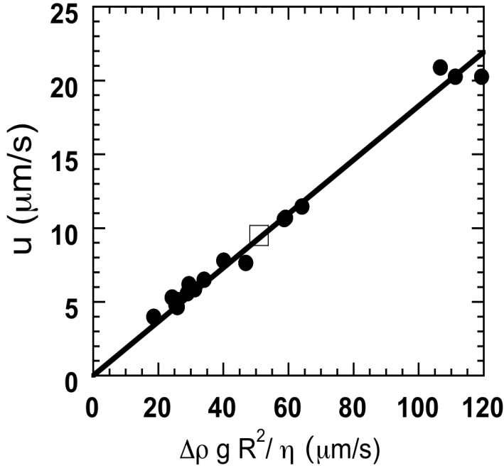
Figure 4. Variation of the translation velocity observed for different vesicles in the steady state versus \Delta\rho g R^2 / \eta , square: velocity of an agarose rigid bead ( R= 36 \mu\text{m} , \Delta\rho=1.0466 ).
