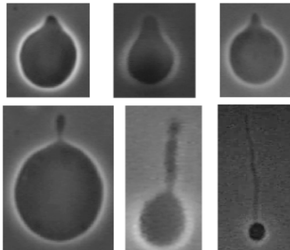
Figure 2 Typical stationary vesicle shapes. Top, pear-like shapes: (1.2) Radius 26 \mu\text{m} , (14.2) Radius 13 \mu\text{m} , (6.2) Radius 32 \mu\text{m} ; bottom, vesicles with tubes: (11.1) Radius 30 \mu\text{m} , (13.1) Radius 16 \mu\text{m} ; Radius 16 \mu\text{m} .
