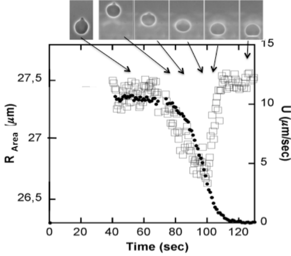
Figure 8: Variation of (A/4\pi)^{1/2} (□) and the velocity (●) versus time. Top: pictures of the vesicle at various times of the sedimentation process.
