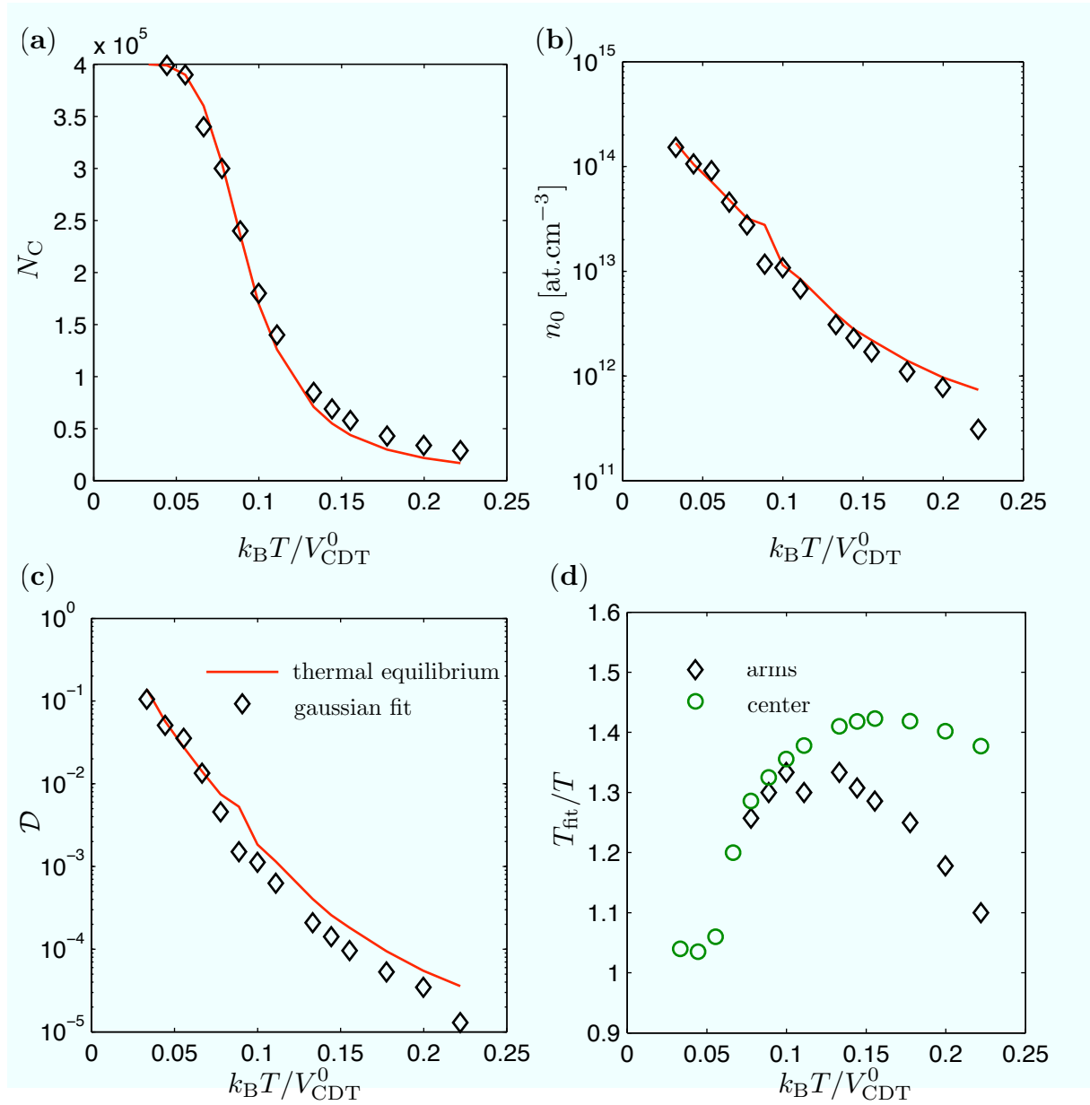
Figure A1. Test of the multicomponent fitting routine used to analyze CDT images. For (a), (b) and (c), black diamonds show the result from the fit. In (a), the center atom number is calculated from the density of states and shown as solid line. For the solid lines in (b) and (c), n_0 and \mathcal{D} are taken from the formulas at thermal equilibrium. In (d), we compare the temperatures extracted from the size of the arms and the size of the central component to the one used for compute the distribution.
