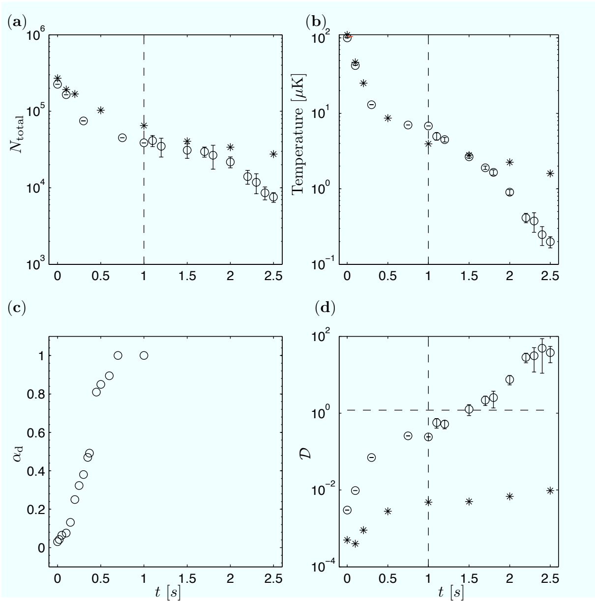
Figure 5. Evaporative cooling trajectories in the combined trap (CDT and dT) (circles) and in the CDT alone (stars). We show the time evolution of atom number N (a), temperature T (b), dimple filling \alpha_d (c) and phase-space density \mathcal{D} (d).
