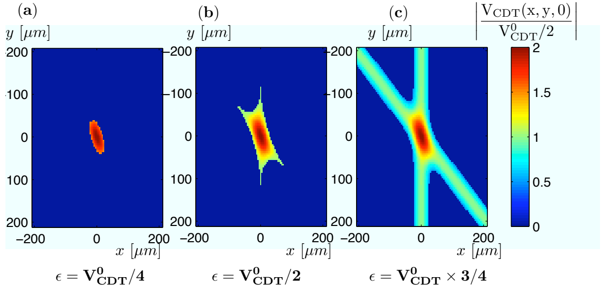
Figure 2. CDT potential in the z = 0 plane, truncated at an energy \epsilon = V_{\text{CDT}}^0/4 (a), \epsilon = V_{\text{CDT}}^0/2 (b), and \epsilon = V_{\text{CDT}}^0 \times 3/4 (c).
