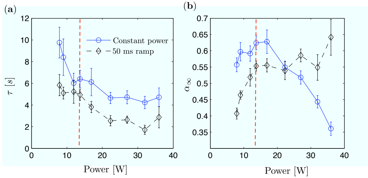
Figure 4. (a) Filling time \tau and (b) center filling fraction \alpha_\infty for CDT in two different situations: the solid curve shows the results of the experiments where the CDT laser is hold at any time at the same power. The dashed curve denotes the compression experiments where the power starts at P_{\text{CDT}} = 13.7 W in the “cold MOT” phase and is ramped up in 50 ms to the final value indicated after switching off the molasses beams. The error-bars correspond to 90% confidence bounds on the fit coefficients \tau and \alpha_\infty . For P_{\text{CDT}} = 13.7 W, both curves should intersect as the experimental sequence is the same. The observed difference indicates systematic variations between different experimental runs, probably due to dipole trap pointing fluctuations and total atom number variations. The vertical dashed line corresponds to the optimal power P_{\text{CDT}} = 13.7 W for the “cold MOT” phase.
