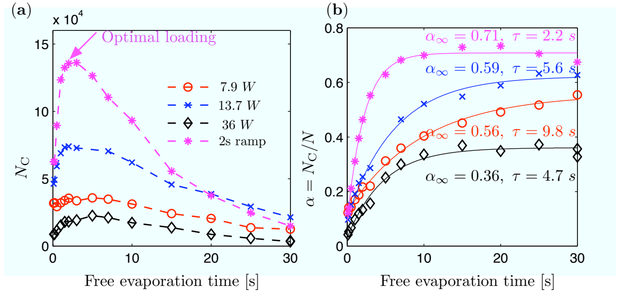
Figure 3. Evolution of the atom number in the center of the CDT (a) and the loading ratio \alpha = N_C/N (b) in four different loading situations: low power (circles), highest power (diamonds), \sim 1/3 of maximum power (crosses), ramping up in 2 s after loading at low power (stars). The loading ratio \alpha(t) is fitted with the function a(1 - e^{-t/\tau}) + b . The results of the fit \tau and \alpha_\infty = a + b are indicated in (b).
