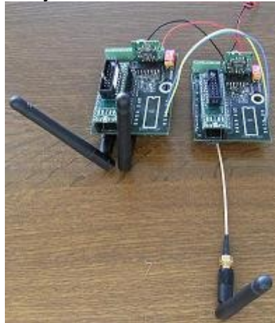
Fig 1: The combination of two LiveNode wireless sensor nodes
