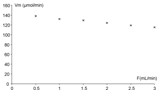
Fig. 3. V_m ( \mu mol/min) vs. the flow-rate A (mL/min). Mobile phase A: 0.1 mM Tris-HCl buffer pH=7.4–10 mM MnCl 2 . Mobile phase B: phosphate buffer (pH=7.00, 50 mM)-methanol (50/50) (v/v)/flow-rate: 3 mL/min. Detection wavelength: 372 nm. IMER temperature: 298 K.
