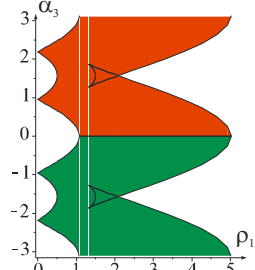
Figure 5: A slice of the joint space for \alpha_2 = \arcsin(1/6) with 2 Q-aspects
