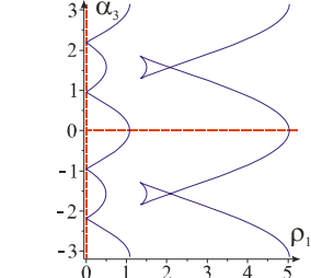
Figure 3: The joint space analysis for \alpha_2 = \arcsin(1/6) with in blue the parallel singularities and in red the serial singularities
