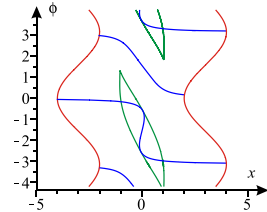
Figure 7: The joint space analysis for \alpha_2 = \arcsin(1/6) with in red the serial singularities, in blue the parallel singularities and in green the characteristic surface
