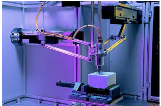
Figure 2: The Orthoglide
