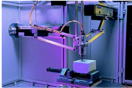
Figure 2: The Orthoglide
