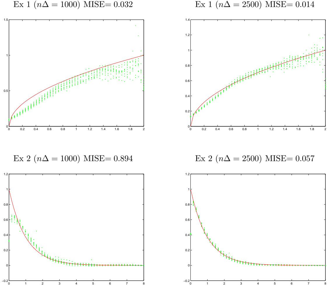
FIGURE 1. Function g (solid line) and estimators \hat{g}_h (dotted lines).
