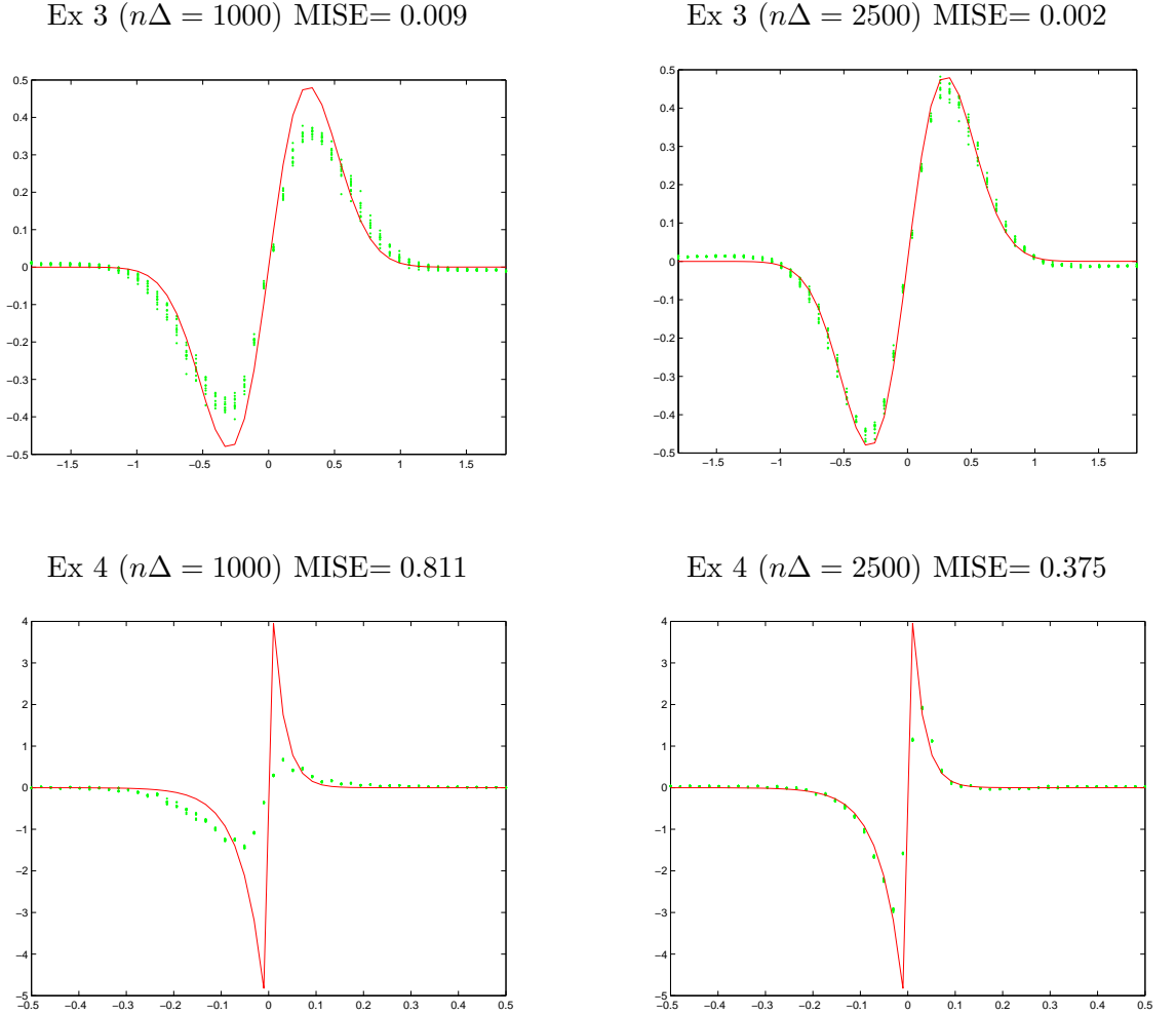
FIGURE 2. Function g (solid line) and estimators \hat{g}_h (dotted lines).
