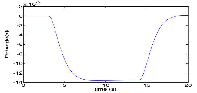
Fig. 8. Pitch angle
