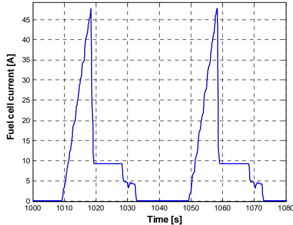
Figure 13 fuel cell current (J227 current profile)
