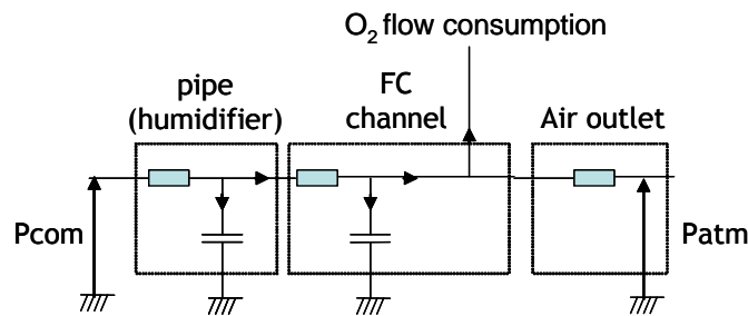
Figure 6 model adopted for the air line
