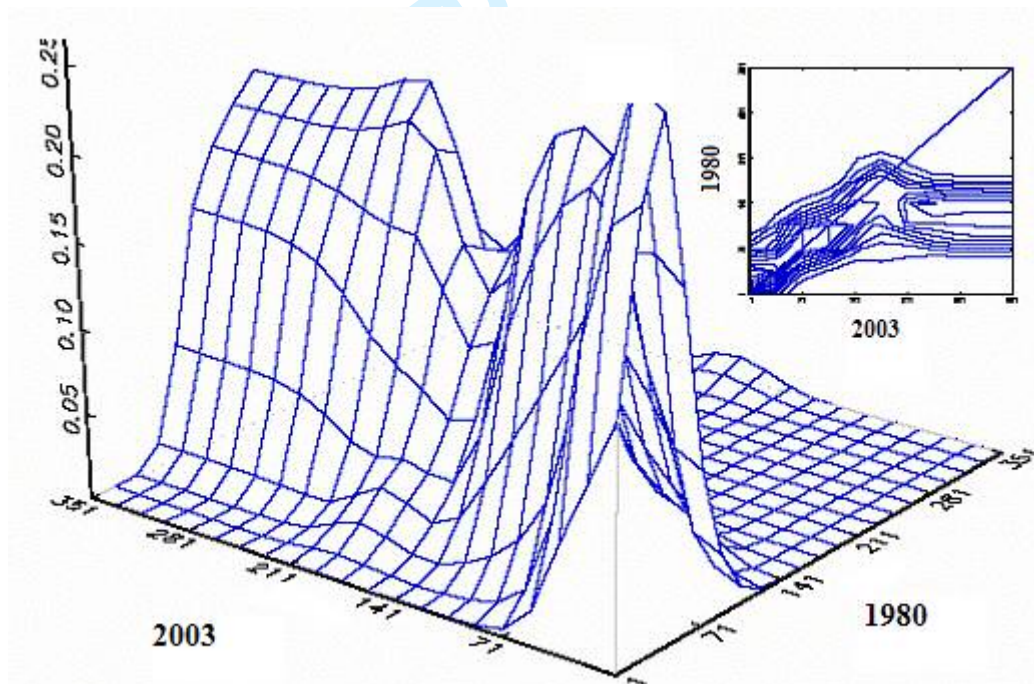
Fig. 3. Stochastic kernel of aggregate productivity
