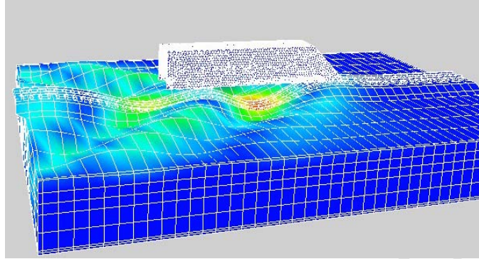
Figure 11a. Wave propagation after a distance of 57 m.
