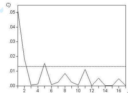
Figure 1: Time decomposition of the Granger causality of CSI for (a) total consumption, (b) consumption of durables (c) consumption of nondurables and (d) consumption of services. The dotted line gives the 5% critical value.
