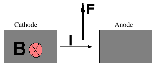
Fig. 6: Sample geometry used during the electrical tests
