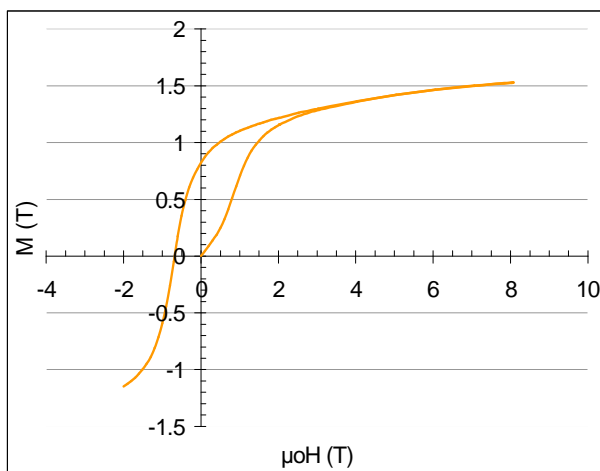
Fig. 4 : M=f(\mu_0 H) for magnetic phase in electrical contact material
