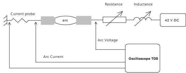
Fig. 5: Electrical test apparatus for break arc
