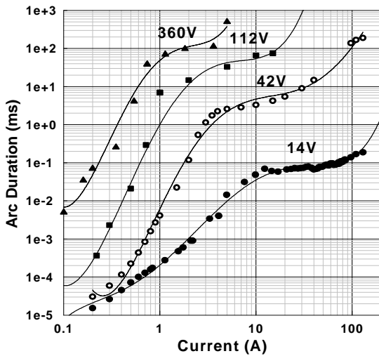
Fig. 1: Arc duration versus current in a range from 0.1 to up to 100A at four circuit voltage (14, 42, 112 and 360VDC)
