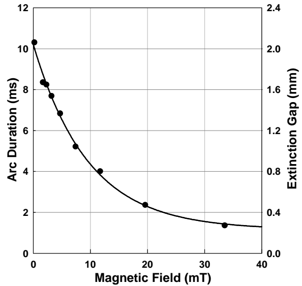
Fig. 3: Arc duration and extinction gap versus external magnetic field for Ag at 42VDC, 37.5A at 20cm/s
