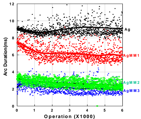
Fig. 10: Arc duration versus number of break operations for Ag, AgMM1, AgMM2 and AgMM3 at 20cm/s 42VDC, 37.5A at 20cm/s
