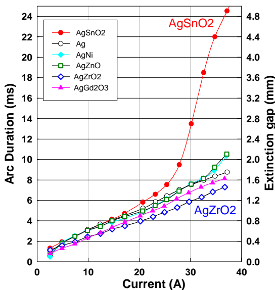
Fig. 2: 42VDC resistive, t=f(I) , Ag, AgNi, AgSnO 2 , AgZnO, AgGd 2 O 3 , AgZrO 2
