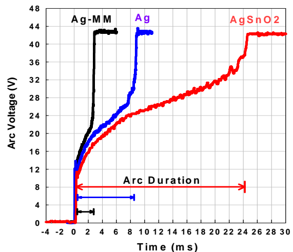
Fig. 7: Arc voltage versus time for AgSnO_2 , Ag and AgMM3 at 42VDC, 37.5A resistive
