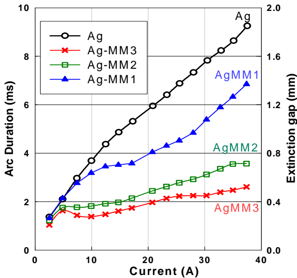
Fig. 8: Arc duration versus Current for Ag, AgMM1, AgMM2 and AgMM3 at 20cm/s 42VDC resistive
