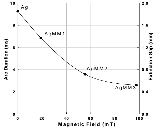
Fig. 9: Arc duration versus Magnetic field for Ag, AgMM1, AgMM2 and AgMM3 at 20cm/s 42VDC, 37.5A at 20cm/s
