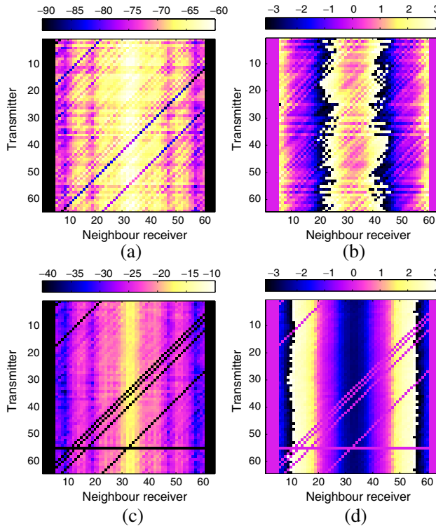
Figure 8. (a) Amplitude in dB and (b) phase of the raw scattering matrix \tilde{\mathbb{K}}_{d,ref}^{meas} . (c) Amplitude in dB and (d) phase of the calibrated scattering matrix \tilde{\mathbb{K}}_{d,ref}^{meas,cal} . The target is the reference target, a centered metallic cylinder with a 90 mm diameter.
