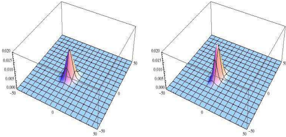
Figure 11: n = 50 ; \beta = 0 , \beta = 1/2
