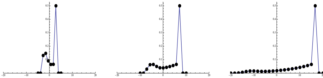
Figure 4: \beta = 1/3 , n=5 , n=10 , n=20
