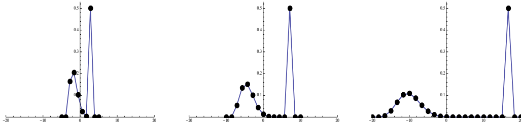
Figure 2: n=5 , n=10 , n=20
