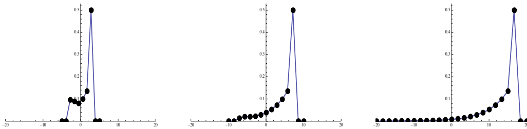
Figure 5: \beta = 1/2 , n=5 , n=10 , n=20
