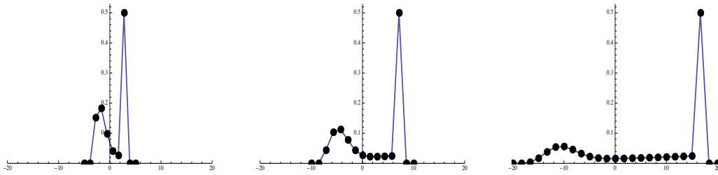
Figure 3: \beta = 1/5 , n=5 , n=10 , n=20
