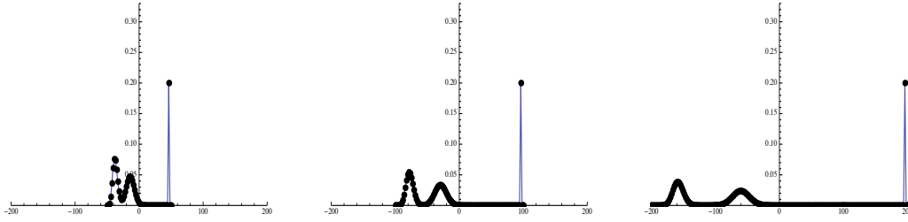
Figure 8: t = 6\pi/40 ; n=50 , n=100 , n=200
