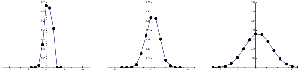
Figure 1: n=4 , n=8 , n=20
