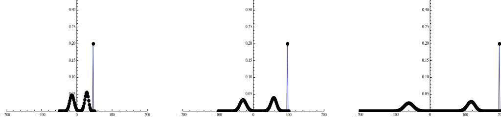
Figure 7: t = 3\pi/40 ; n=50 , n=100 , n=200
