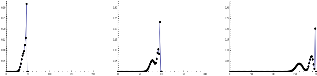
Figure 6: t = \pi/40 ; n=50 , n=100 , n=200
