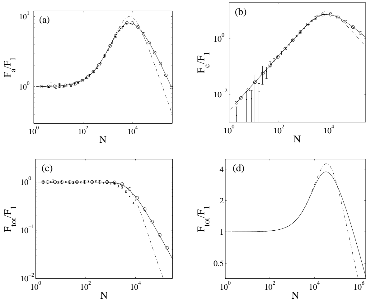
FIG. 1: (a) Absorption, (b) emission and (c) total forces vs N for \delta = 10 and a Gaussian cloud with \sigma = 8 . (d) Total force for \sigma = 5 and \delta = 200 . Forces are relative to the single-atom force F_1 . The plain curves refer to the series (35), (36) and their sum, the circles to the analytical expressions (46), (36) and their sum, the dots to N -body simulations (see Eq.4) and the dash-dotted lines to the STD state. The error bars correspond to the standard deviation of the observables over 8 realizations.
