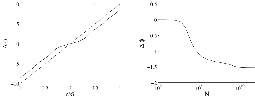
FIG. 4: Left: Phase shift along the optical axis for the exact solution (15) (plain line) and a STD state (49) (dash-dotted line). Right: Phase shift of the pump beam after transmission through the cloud as a function of N evaluated along the axis, x = y = 0 , at k_0 z = 20\sigma , for N = 10^4 , \sigma = 10 and \delta = 10 .
