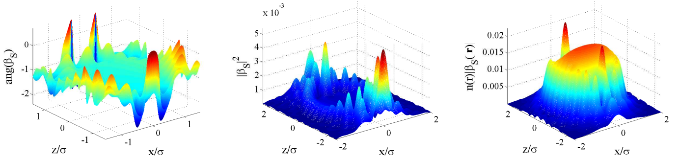
FIG. 3: Phase of the atomic radiation \text{ang}(\beta_s) (left), Excitation probability |\beta_s|^2 of the atoms in the (x, z) plane ( y = 0 ) (center) and contribution to the radiation of the electric field in the same plane, which corresponds to the level of excitation of the atoms weighted by their local density (right). Simulations realized using the analytic expressions (15), for N = 10^4 , \sigma = 10 and \delta = 10 .
