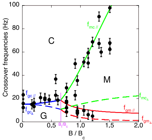
FIG. 4: (color online). Crossover frequencies f_{gc} , f_{gm} and f_{mc} ( \bullet ) as a function of the horizontal magnetic field B/B_c . Solid lines f_{gc\parallel} (middle blue line), f_{gm\parallel} (lower red line), and f_{mc\parallel} (upper green line) are from Eqs. (4), (5) and (6) respectively. The triple point ( f_t = 18.7 Hz, B_t/B_c = 0.65 ) is from Eq. (7). Dashed lines correspond to the theoretical crossovers f_{gc\perp} , f_{gm\perp} and f_{mc\perp} for the normal field case [6]. Forcing parameters: 1 - 6 Hz. B_c = 294 G.
