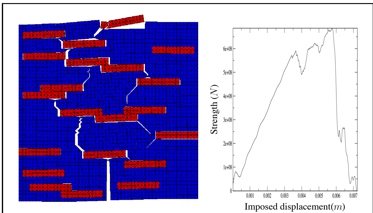
Figure 2. Weak matrix/hydrides interface.
