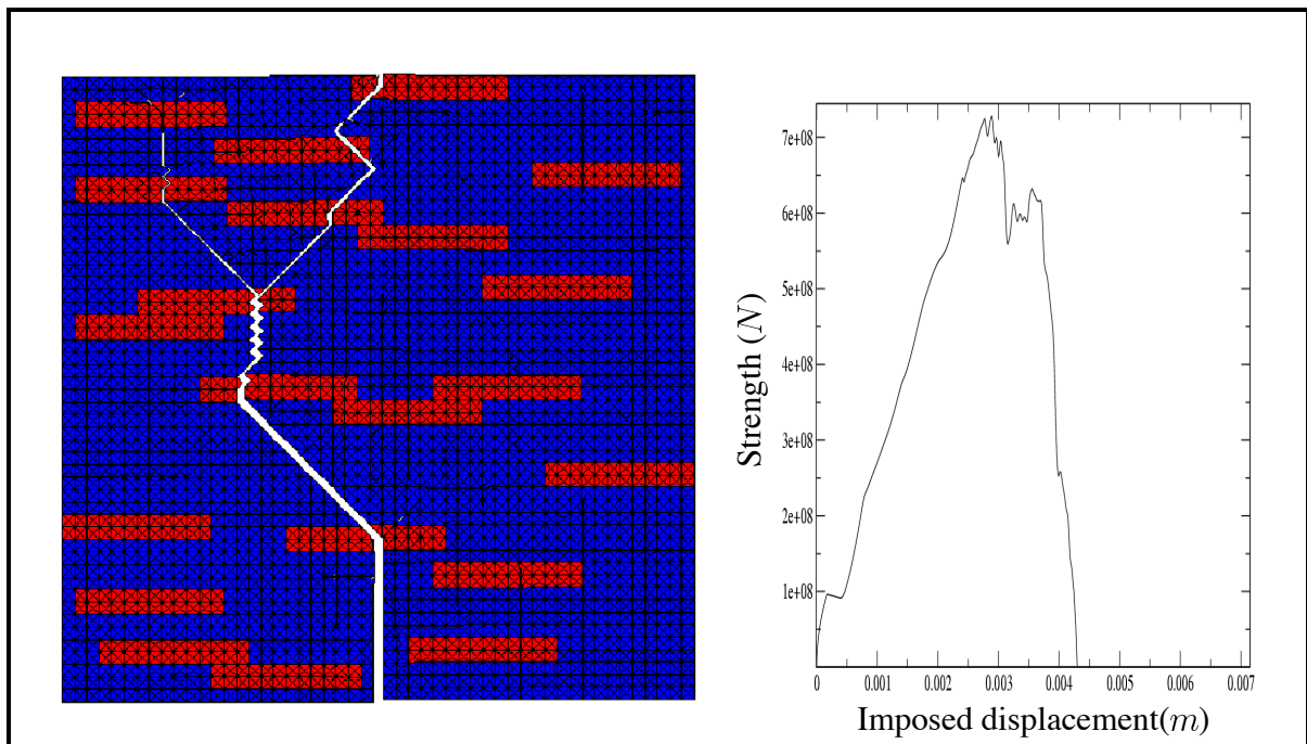
Figure 1. Strong matrix/hydrides interface.
