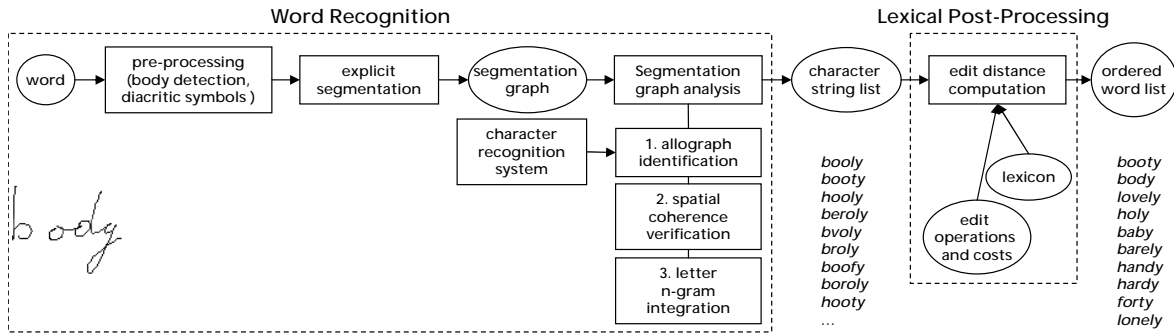
Figure 1. Word recognition system.
