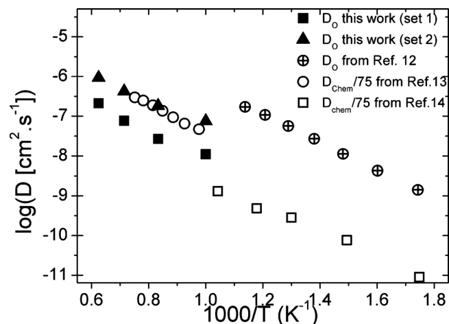
FIG. 1. Arrhenius plot of oxygen diffusivity in \text{GdBaCo}_2\text{O}_{5.5} : simulations (triangles) and comparison to diffusion coefficient as obtained from oxygen exchange (Ref. 12) and from oxygen chemical diffusion oxygen corrected by thermodynamic factor (Refs. 13 and 14).
