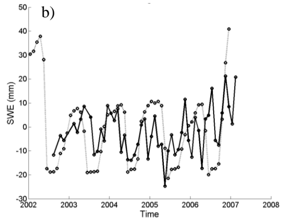
Figure 6: Time series of SWE (mm) derived from GRACE (black) and WGHM (dotted black) for the Nelson (a) and Indigirka (b) basins.
