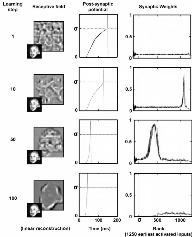
Fig. 3. One STDP neuron learns one V1-filtered image (here, Einstein's face). (Right column) Synaptic weights. Affereents are ordered with increasing latencies. Notice how STDP tracks back through the spike train, depressing synapses it had previously reinforced, until having concentrated all the weights on the earliest firing afferents. The final number of selected afferents depends on the threshold \sigma . (Middle column) Postsynaptic membrane potential as a function of time. Notice how the postsynaptic spike latency decreases as learning progresses (Left column) Linear reconstruction of the neuron's preferred stimulus. Before learning, since the synaptic weights are random, so is the reconstruction. But after learning, the neuron became selective to the most salient edges of the input image. Reproduced with permission from [26].
