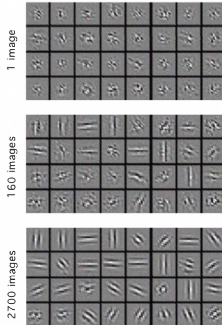
Fig. 6. Pattern of connectivity of 64 maps of V1 neurons inhibiting each other. The pattern of connectivity of neurons were initialized with two arrays (ON and OFF) of size 11 \times 11 whose synaptic weights were distributed according to a randomized Gaussian function (the reconstruction process display here take into account both of these arrays, synapses from ON-center neurons being counted as positive and those from OFF-center neurons being counted as negative). After propagating thousands of images, coherent receptive fields were found to arise naturally for these 64 maps of neurons. Interestingly, they look like the selectivities found in V1 (reproduced with permission from [49]).
