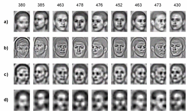
Fig. 5. Receptive fields of all STDP neurons after 4000 learning steps. Images in a) show additive reconstructions from learned weights of all feature channels (scale, orientation and phase polarity). b) - d) Idem, but separated for each Gabor scale from fine to coarse. It is clearly visible that the neurons show a preference for particular head poses. The numbers over each column denote the quantity of learning steps for each neuron (reproduced with permission from [36]).
