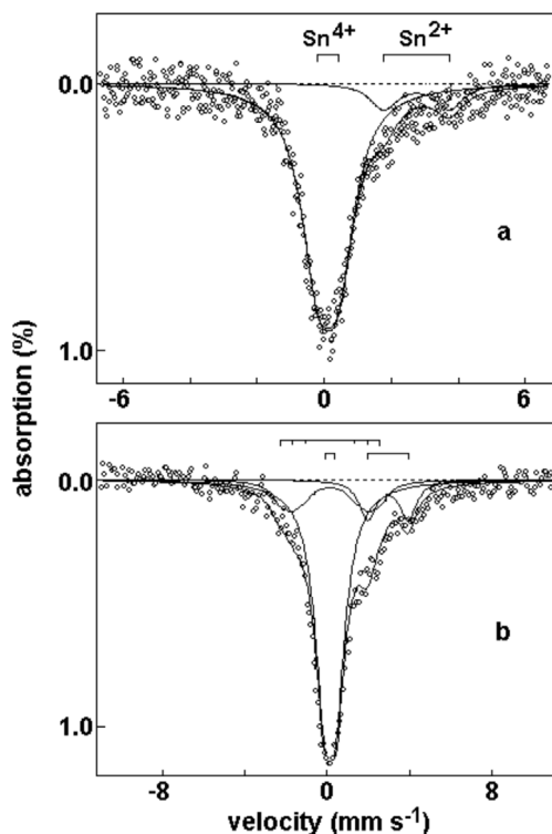
Fig. 4. ^{119}\text{Sn} Mössbauer spectra of sample 2_{\text{ox}} ; T_{\text{meas}} = 295 K (a) and 4.2 K (b).
