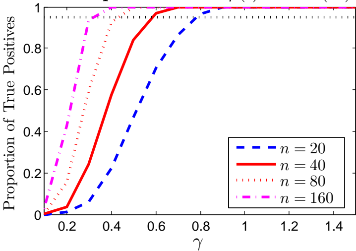
True positive rate \varphi(t) = c \cos(4t)
