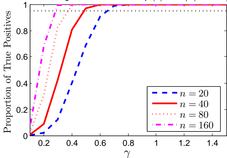
True positive rate \varphi(t) = c/(1+t^2)
