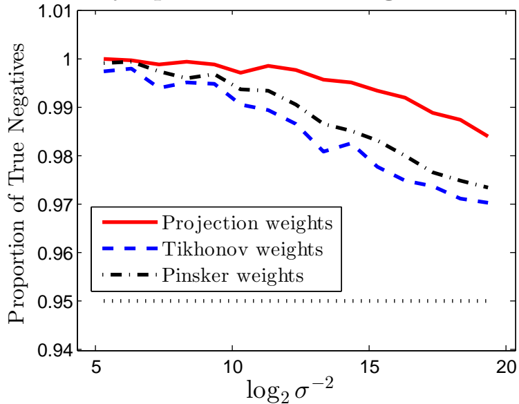
Asymptotics of true negative rate
