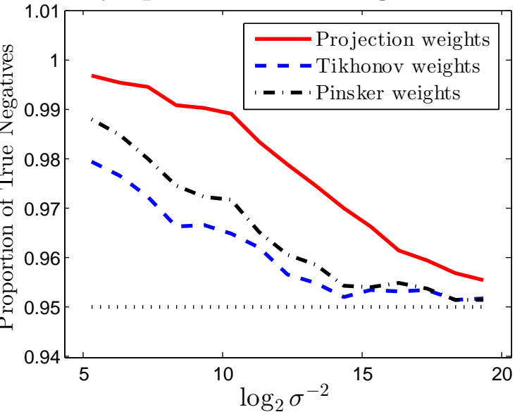
Asymptotics of true negative rate
