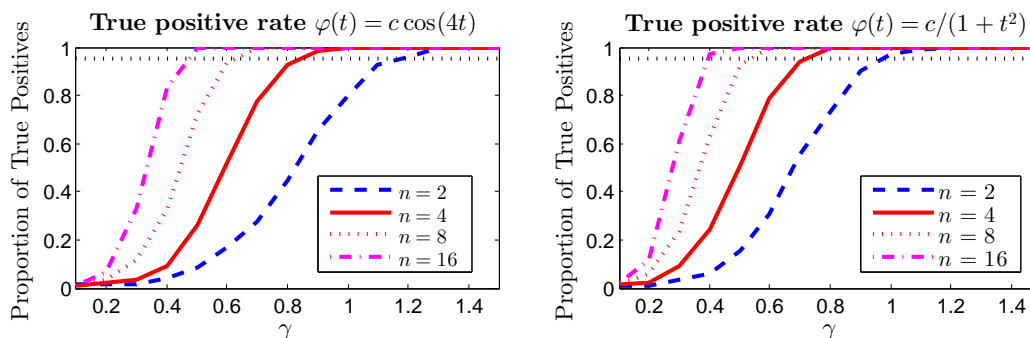
Figure 2: The proportion of true positives in the experiment described in Section 4.2 as a function of the parameter \gamma measuring the “distance” from the null. The parameter n is defined as \sigma_*^{-2} , where \sigma_* is the noise level. We can observe that even for relatively small values of \gamma the test has a power close to one.
