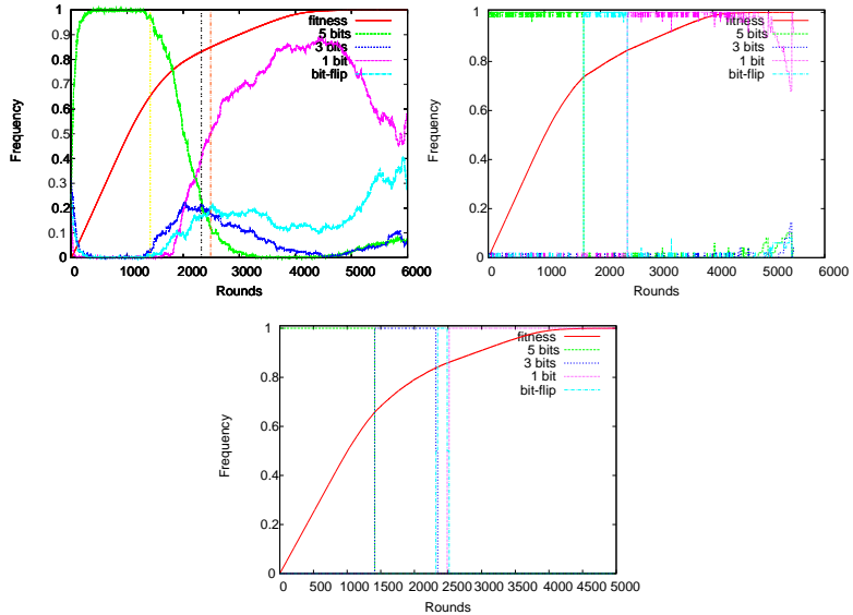
Figure 6: Top left (resp. right): Evolution of the average number of nodes (resp. number of nodes for the median run) of each mutation operator using a complete topology with n = 50 , \lambda = 1 , and p_{mut} = 10^{-3} . Bottom: Evolution of the mutation operator in average according to the sequential oracle with \lambda = 50 .
