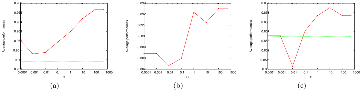
Figure 3: Average fitness found by VEGAS C as a function of C. K = 6 (a) q = 2 (b) q = 3 (c) q = 4 . The horizontal dotted line is the performance of F2NS.
